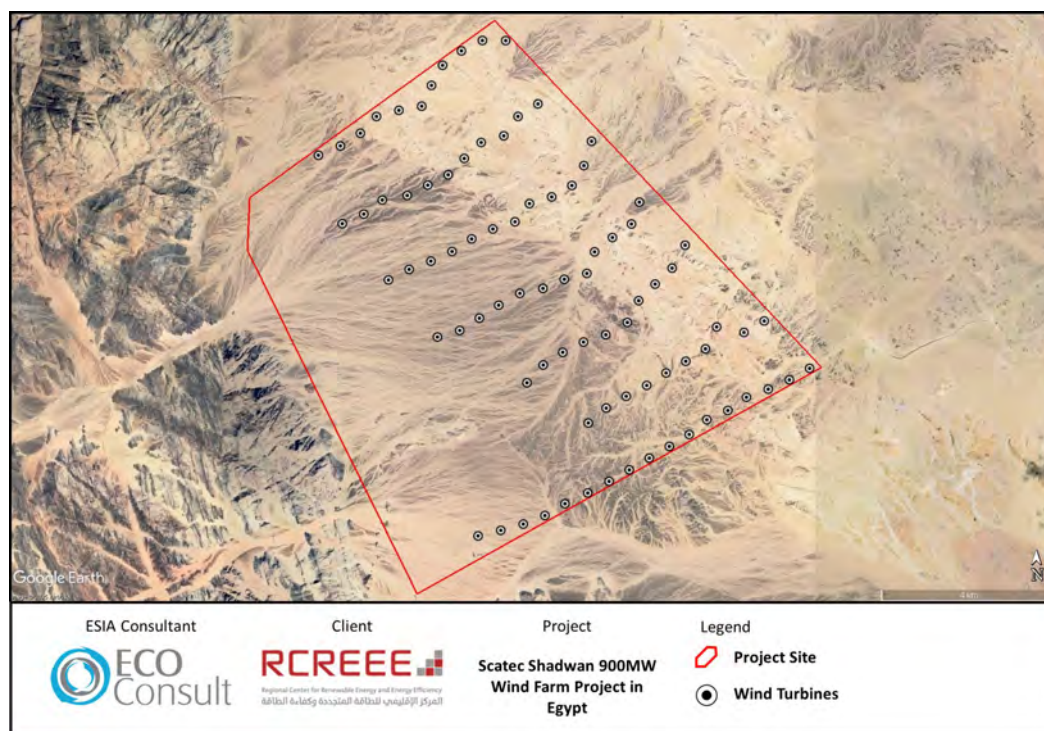
Figure 5: Final WTG Layout
