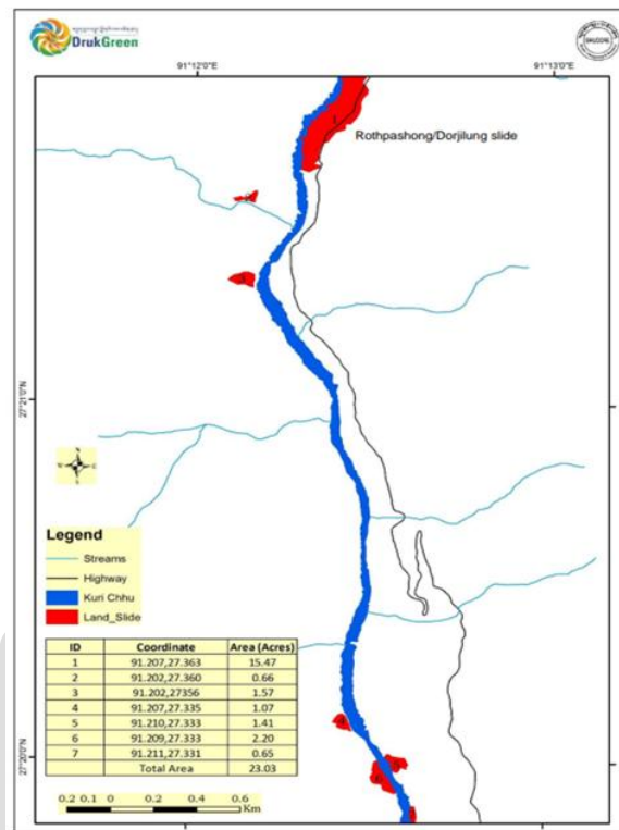
Figure 5: Areas Prone to Landslide
