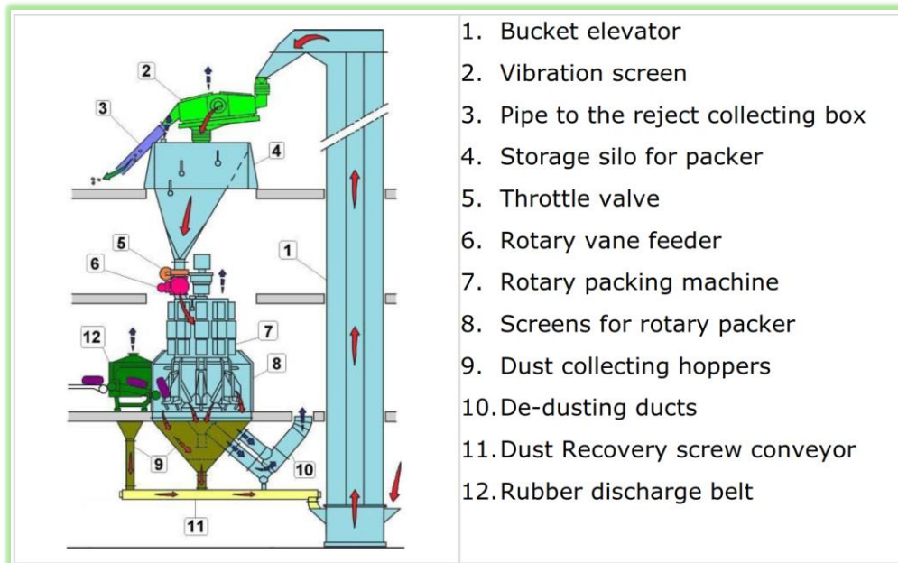
Figure 3-10: Typical packing/bagging plant
