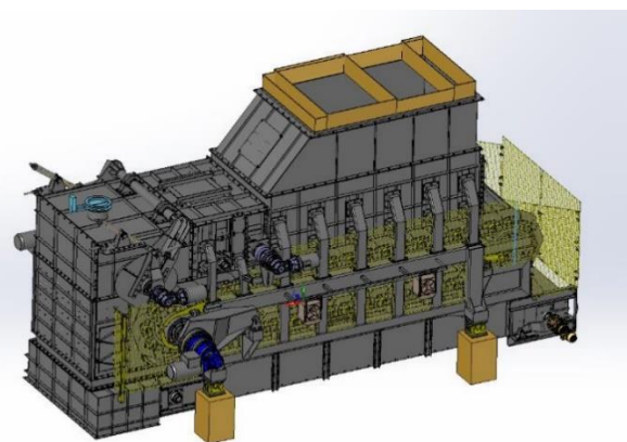
Figure 3-15: Proposed box feeder (left) for the calciner and a 3D Version (right)
