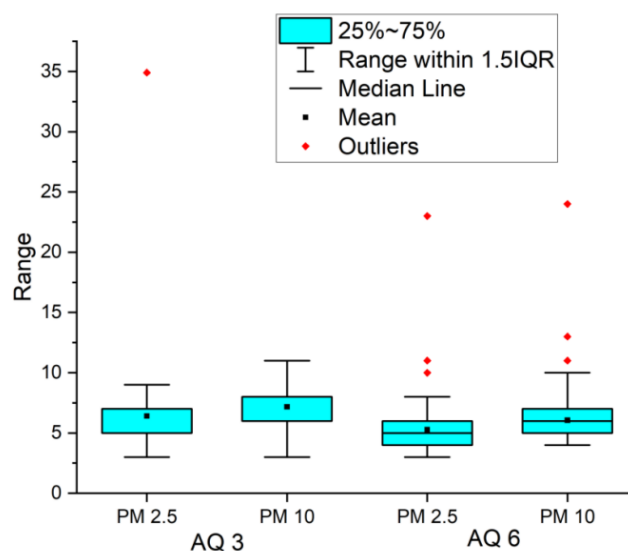
Figure 6.21– Box Plots for Air Quality at Day 3
