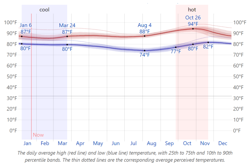
Figure 6.3 – Average high and low temperatures in Manatuto
