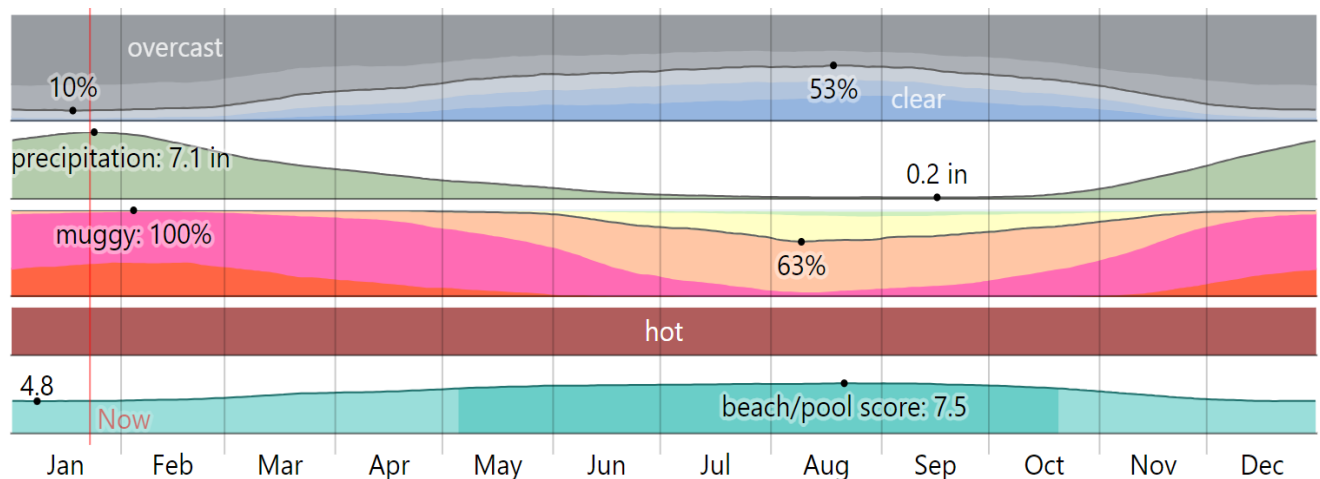
Figure 6.1 – Climate in Manatuto
