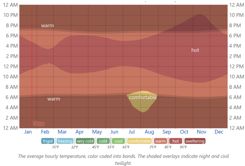
Figure 6.2 – Average hourly temperature in Manatuto
