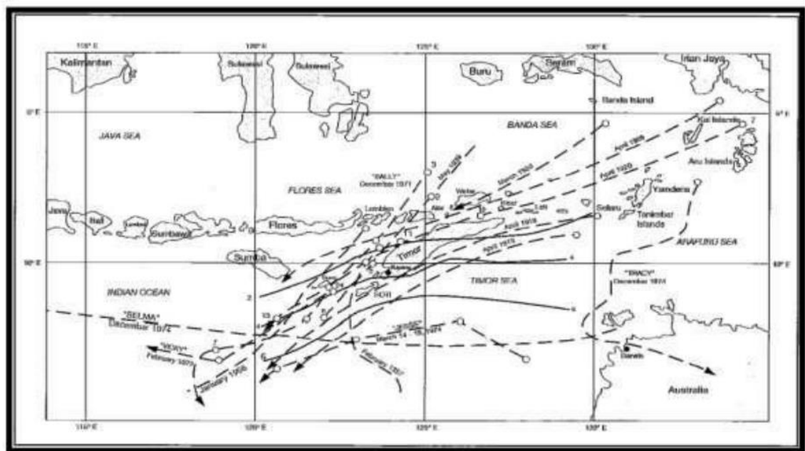
Figure 5: Occurrence of tropical cyclones in the past over Timor-Leste region (Crippen International 10, quoted in Monk et al. 1997).
