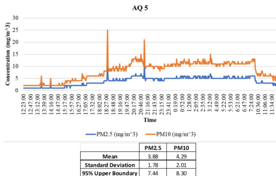
Figure 6.17 – Overall trends in air quality at AQ5
