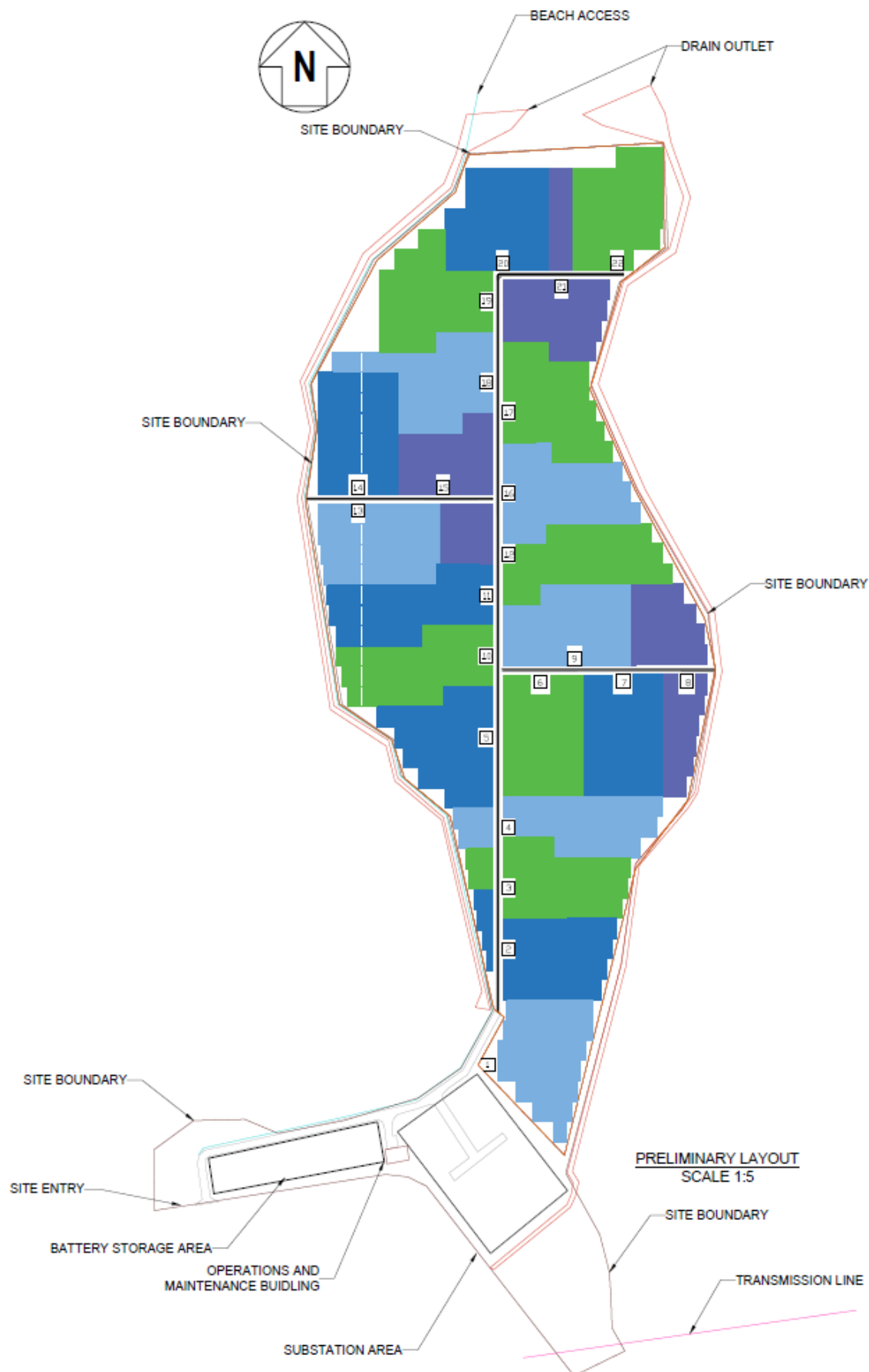
Figure 4.4: Indicative Site Layout
