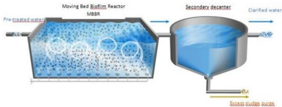
Figure 2: A schematic MBBR
