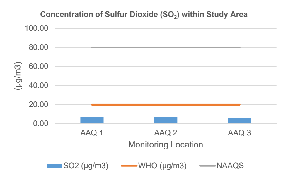
Figure 4.14 Concentration of Sulphur Dioxide (SO 2 ) in the Study Area
