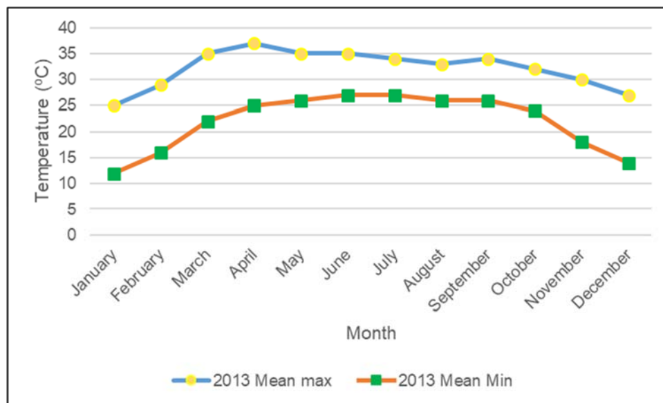
Figure 4.7 Monthly Mean Minimum and Maximum Temperature Variations
