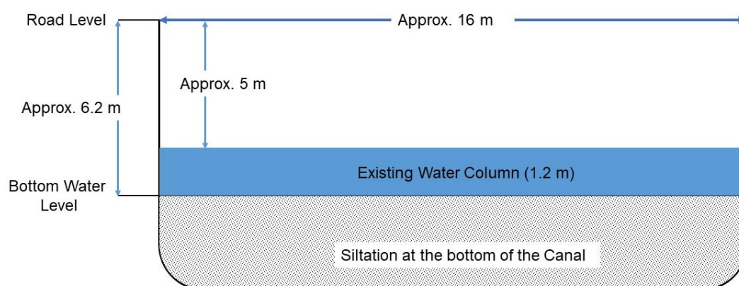
Figure 4.22 Cross-sectional Area of Howrah Drainage Channel
