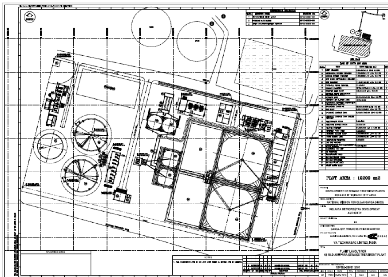
Figure 2.10 Proposed Site Layout of Arupara STP
