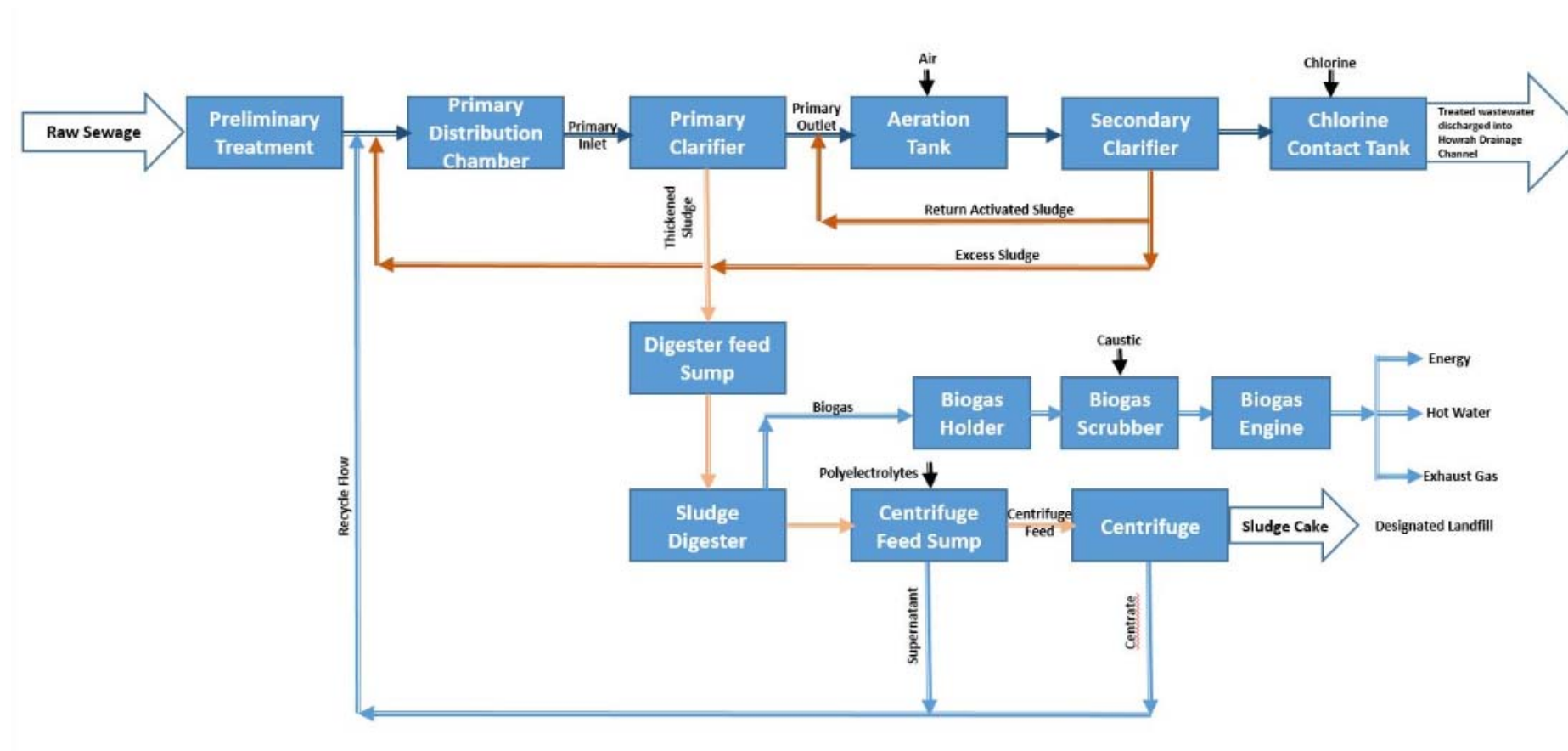
Figure 2.12 Process Block Diagram of Proposed Arupara STP
