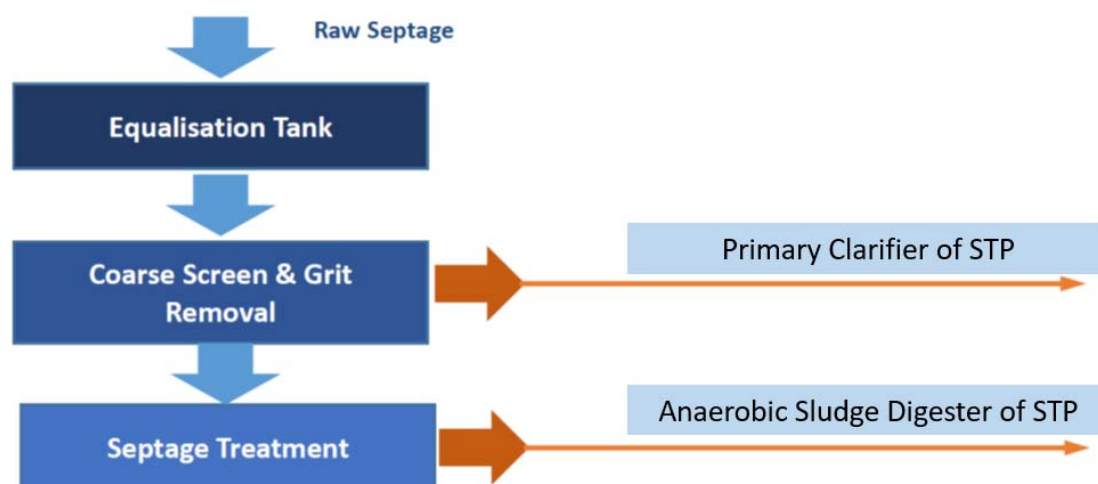
Figure 2.13 Septage Treatment Process Flow
