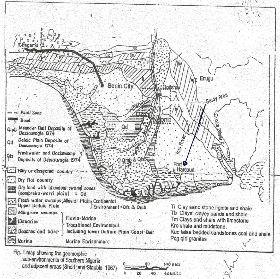
Figure 4.6.1: geologic characteristics of the study area
