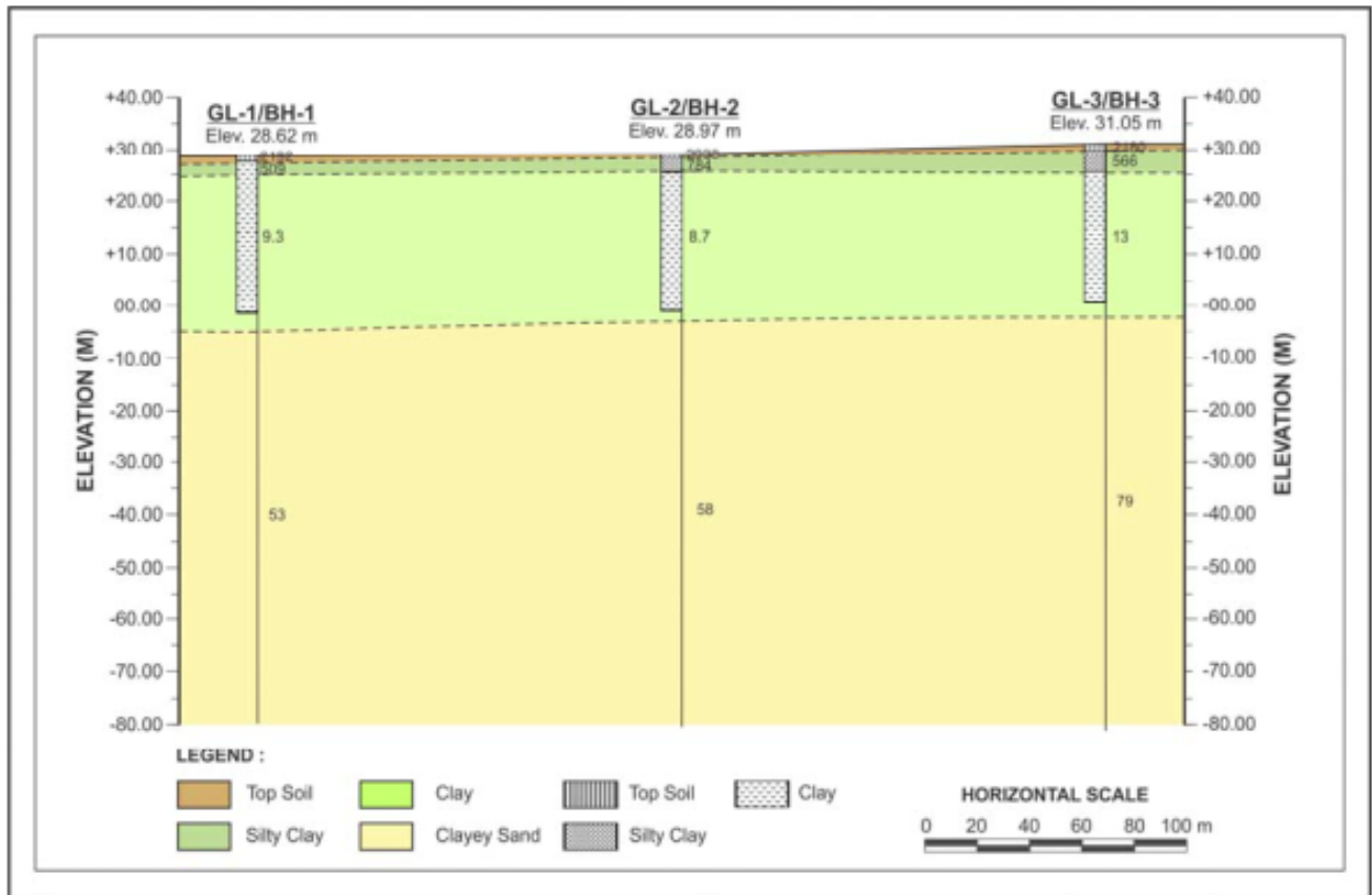
Figure 3.11 : Cross-Section Showing Results of Resistivity Survey
