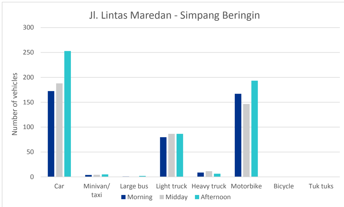
Figure 3.46 : Graph Showing Traffic Counts for Location Two: Jl. Lintas Maredan – Simpang Beringin
