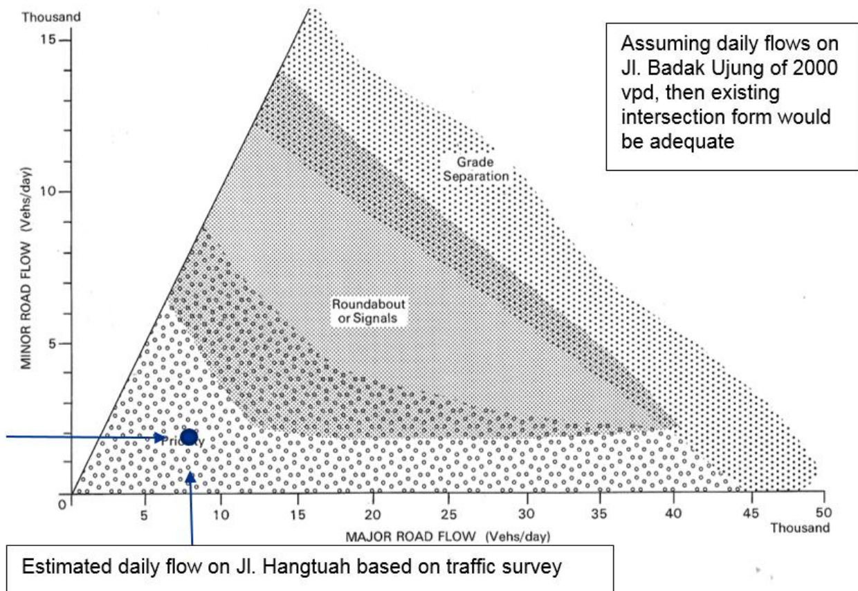
Figure 13.2 : Jl. Hangtuah / Jl. Badak Ujung Intersection Control
