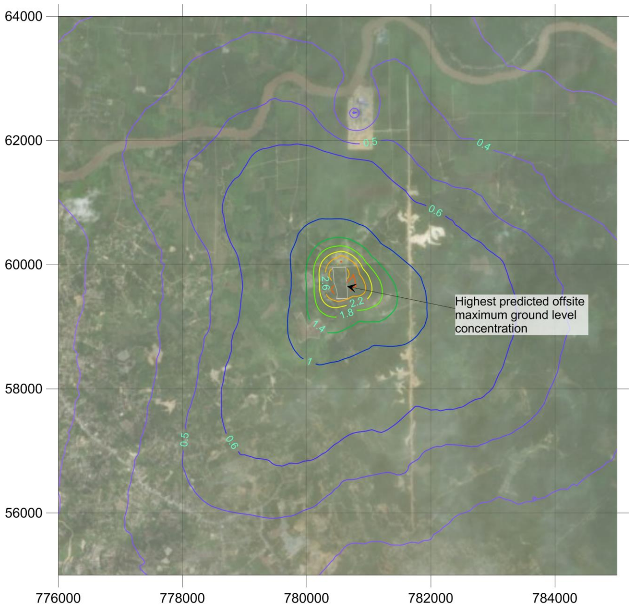
Figure 4.4 : Highest Predicted Maximum Ground Level Concentrations (Annual Average) of NO 2 (µg/m 3 ) from Discharges from the Proposed Power Plant (Excluding Background)
