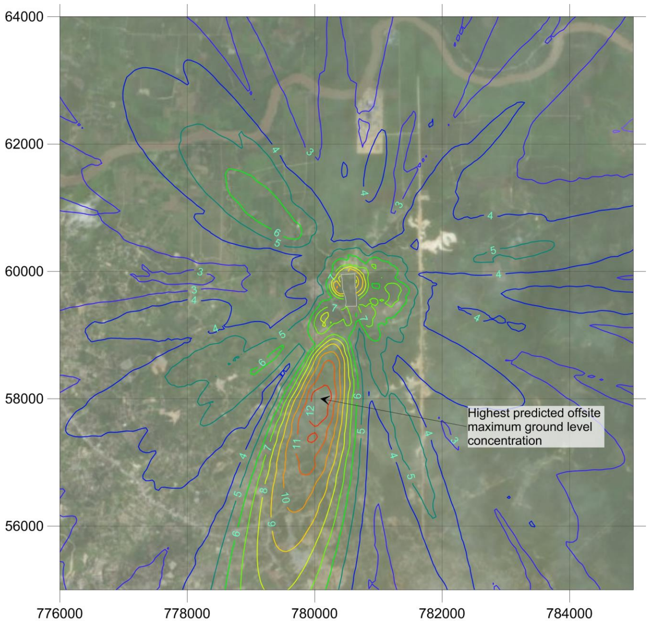
Figure 4.3 : Highest Predicted Maximum Ground Level Concentrations (24-Hour Average) of NO 2 (µg/m 3 ) from Discharges from the Proposed Power Plant (Excluding Background)
