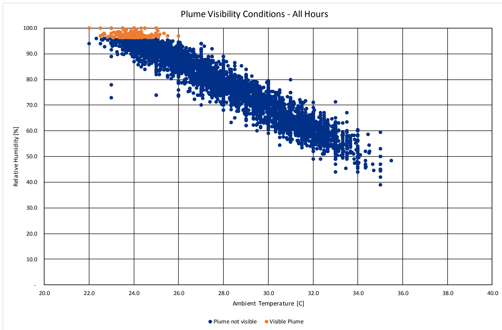
Figure 9.7 : Plume Visibility – 2013 to 2015
