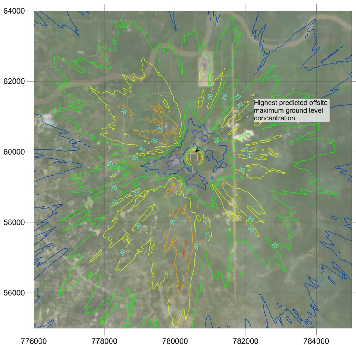
Figure 4.2 : Highest Predicted Maximum Ground Level Concentrations (1-Hour Average, 99.9 th Percentile) of NO 2 (µg/m 3 ) from Discharges from the Proposed Power Plant (Excluding Background)
