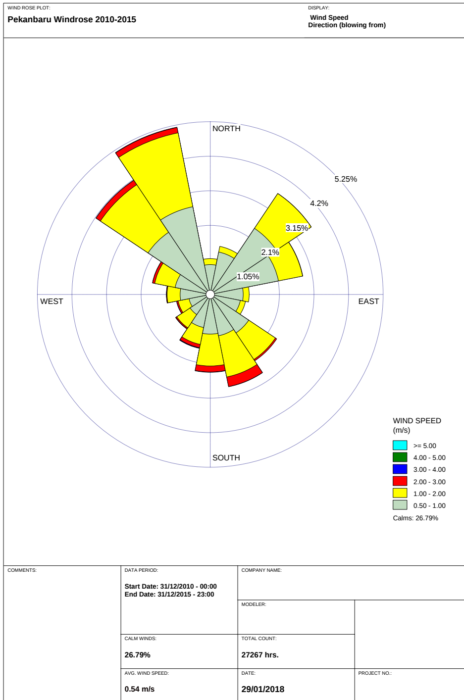
Figure 3.2 : Windrose of Data Collected at Pekanbaru (Years 2010 – 2015)
