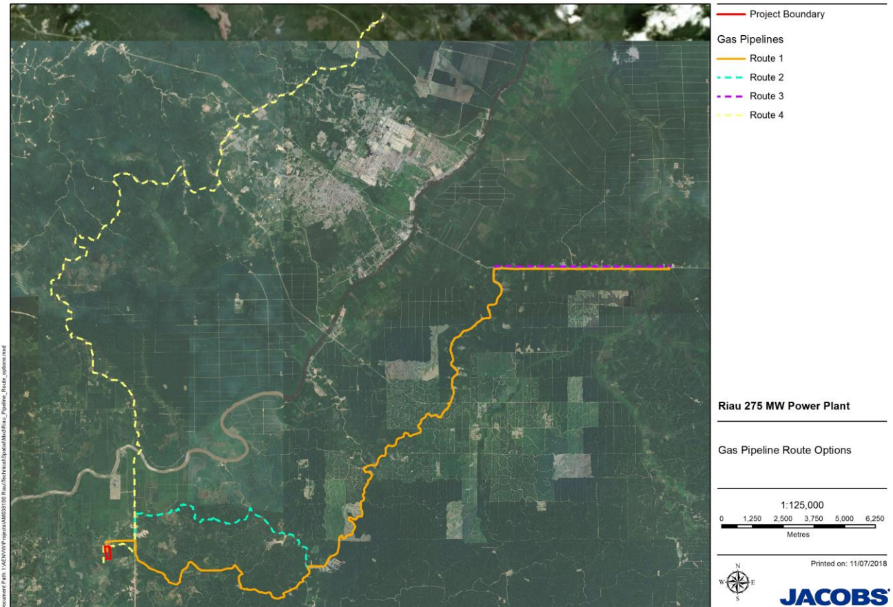
Figure 4.2 : Gas Pipeline Route Options
