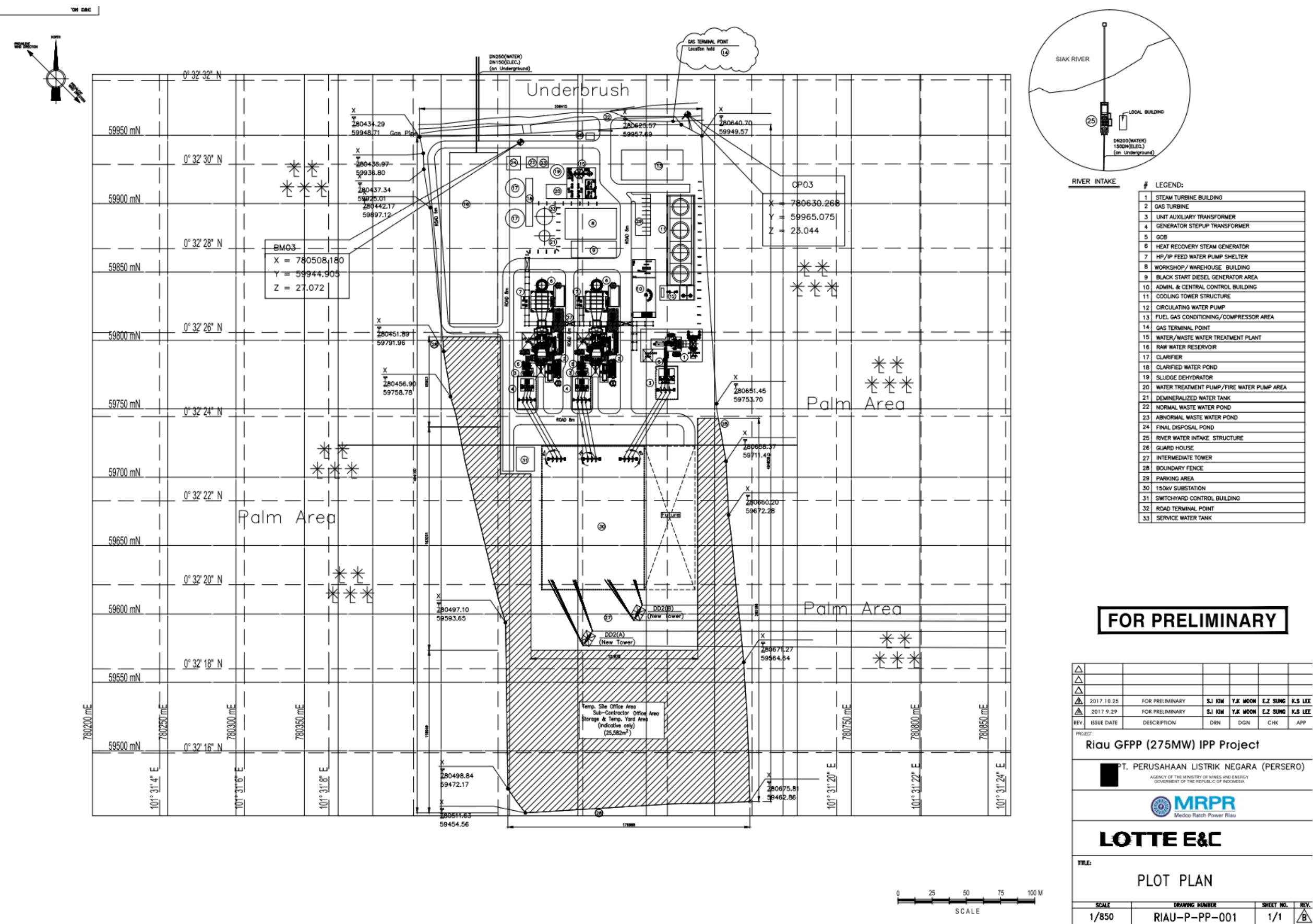
Figure 3.6 : Plot Plan of Power Plant
