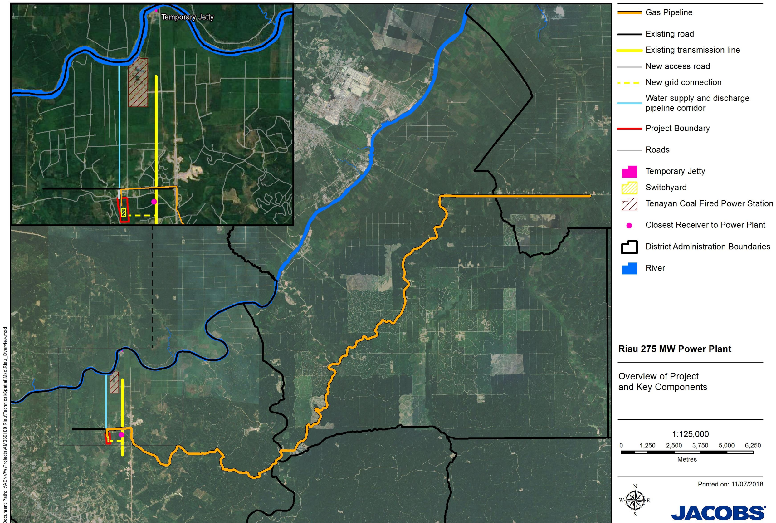
Figure 3.1 : Overview of Project and Key Components
