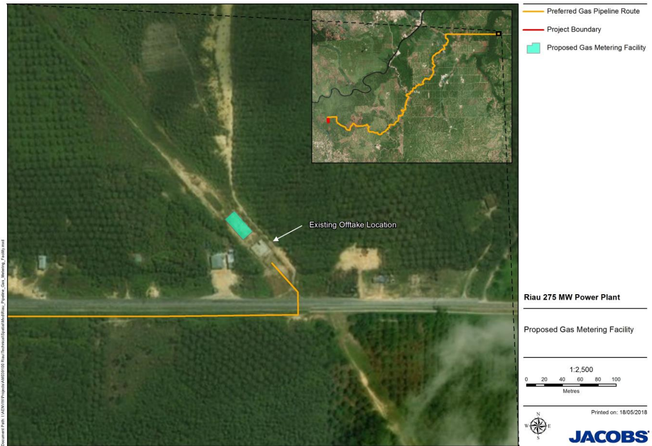
Figure 3.5 : Location of Gas Metering Facility
