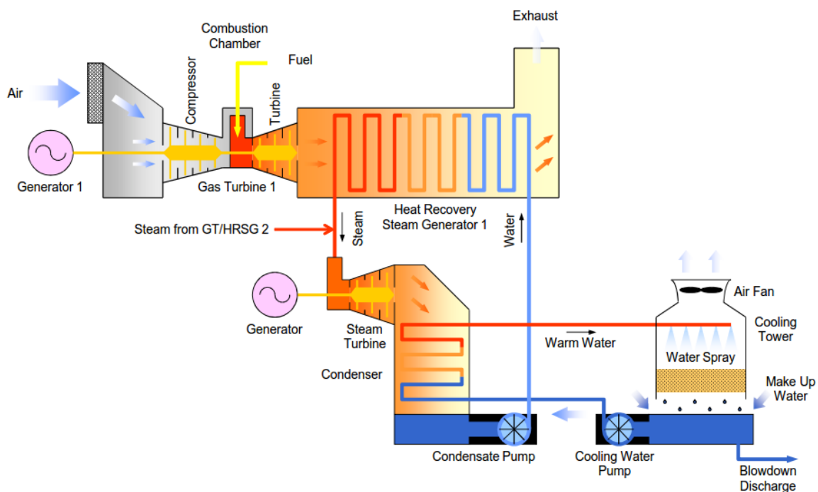
Figure 3.7 : Schematic of General Process
