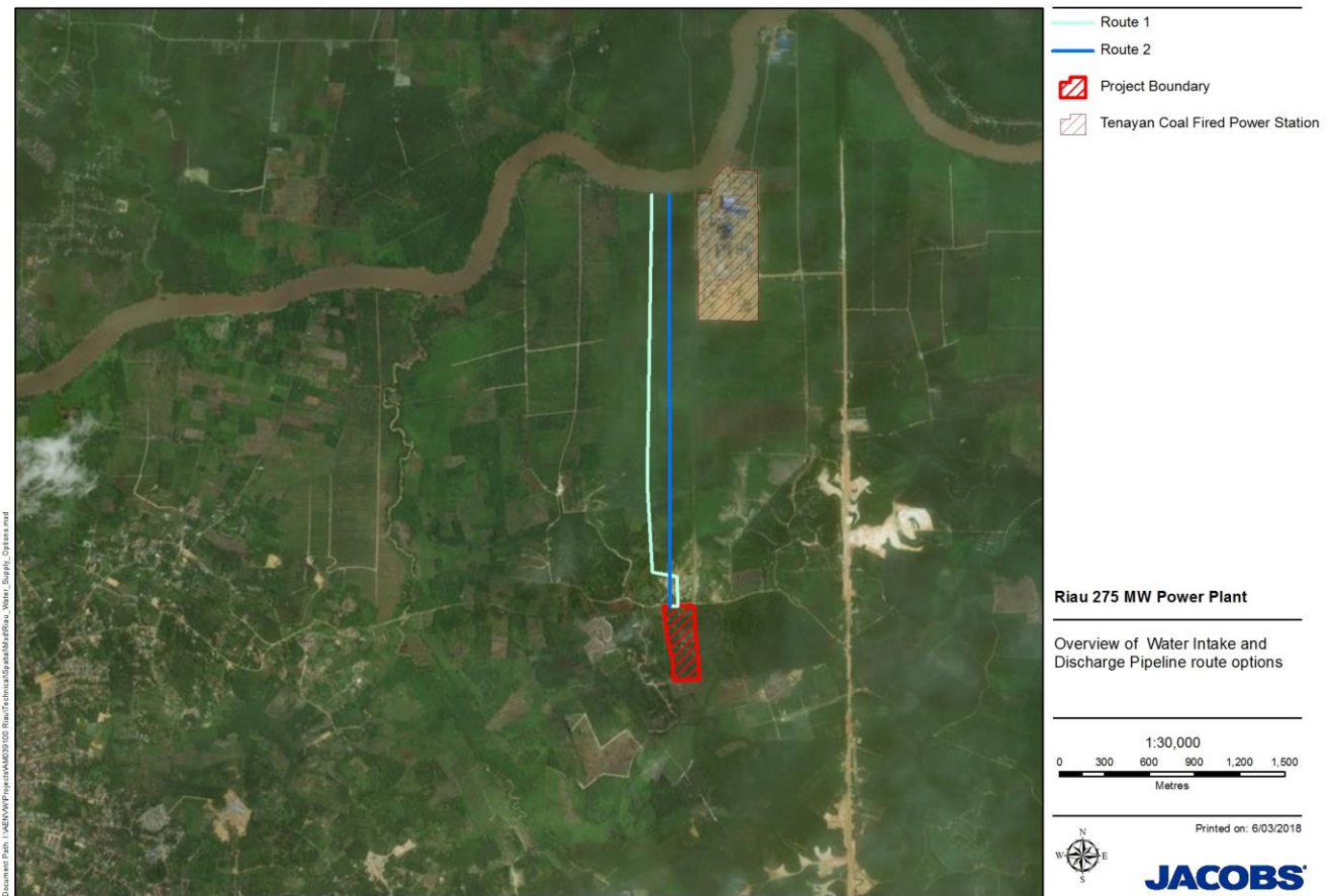
Figure 4.3 : Water Intake and Discharge Pipeline Route Options
