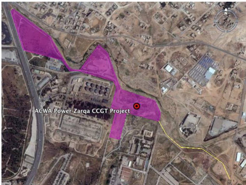
Figure 1-6 NEPCO Pipeline Spur to the ACWA Power Zarqa CCGT Project (routing in yellow)
