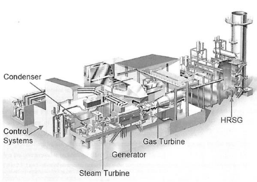
Figure 1-3 Illustration of Typical CCGT Plant
