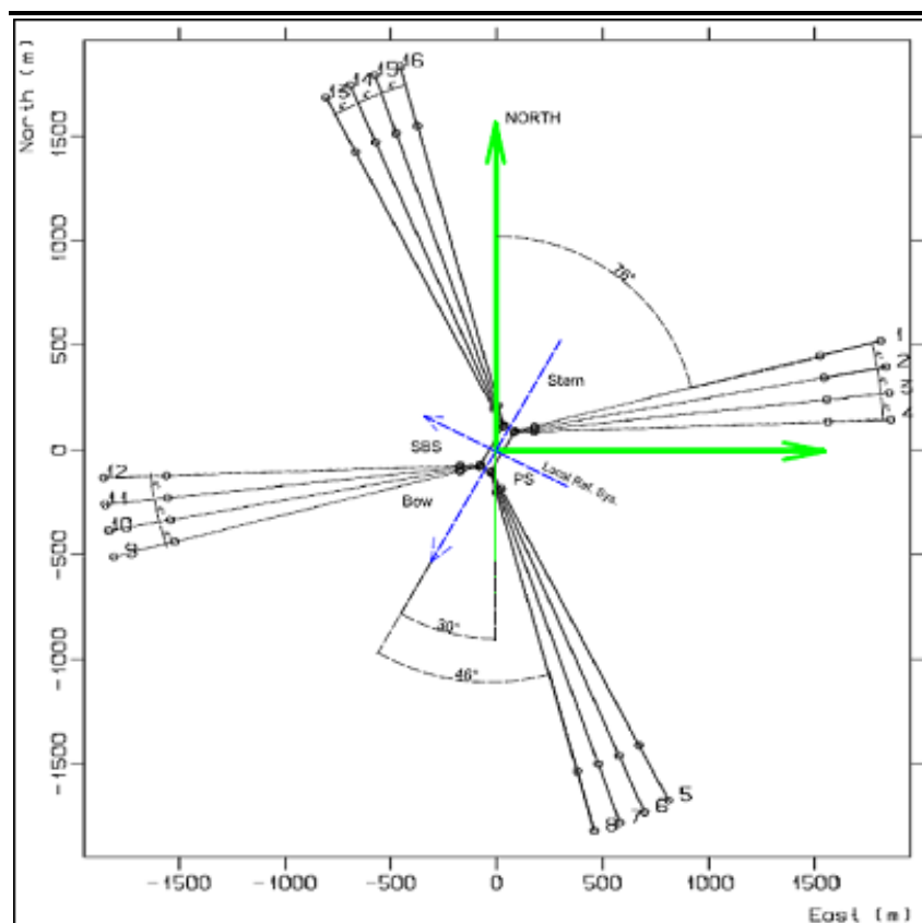
Figure 4.24 FPSO Mooring Pattern
