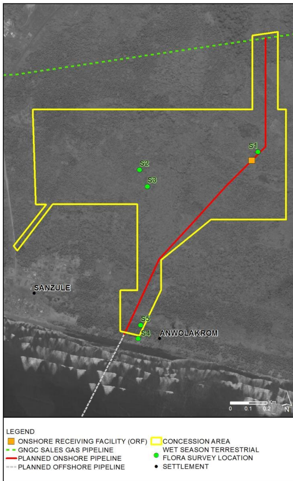
Figure 6.24 Flora sampling locations (wet season)
