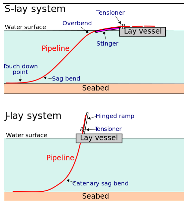
Figure 4.15 S-lay and J-lay methods
