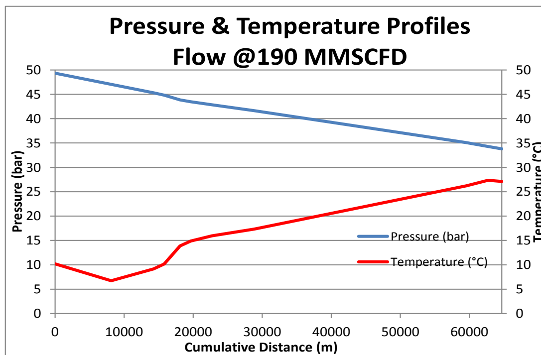
Figure 4.13 Pressure and Temperature profile at 190 MMSCFD
