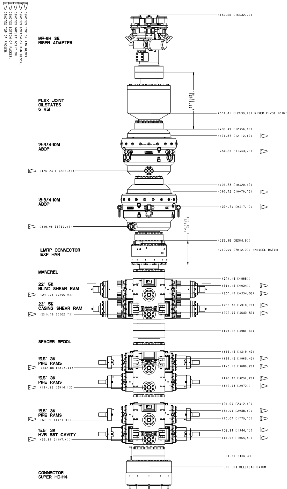
Figure 4.23 BOP stack configuration for Maersk Voyager drilling rig
