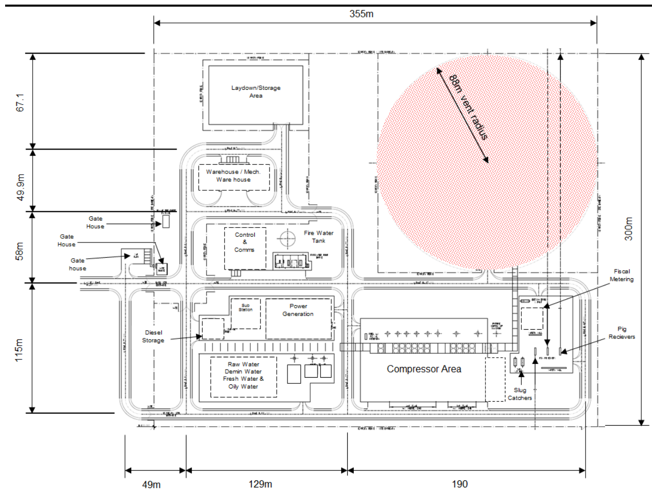
Figure 4.20 ORF Layout
