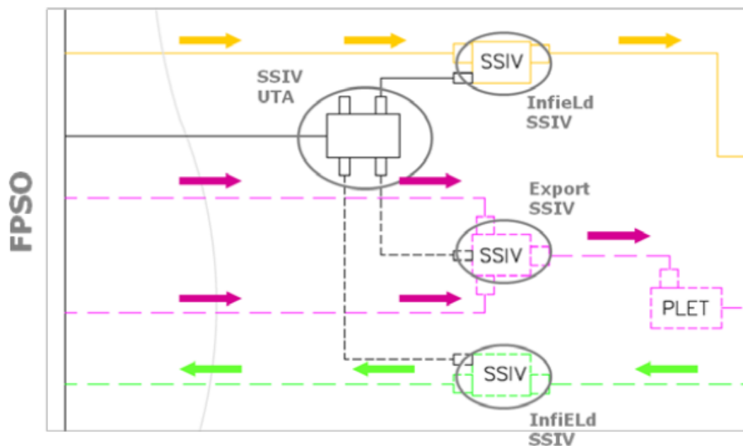
Figure 4.14 Subsea Isolation Valve System
