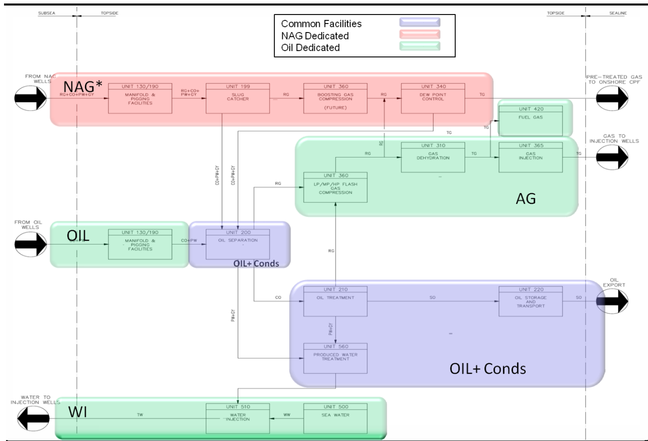
Figure 4.8 FPSO Unit Schematic Layout
