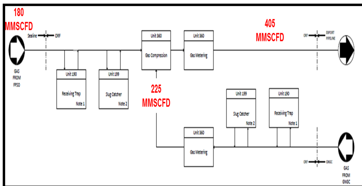
Figure 4.4.19 ORF Aggregate Compression Station
