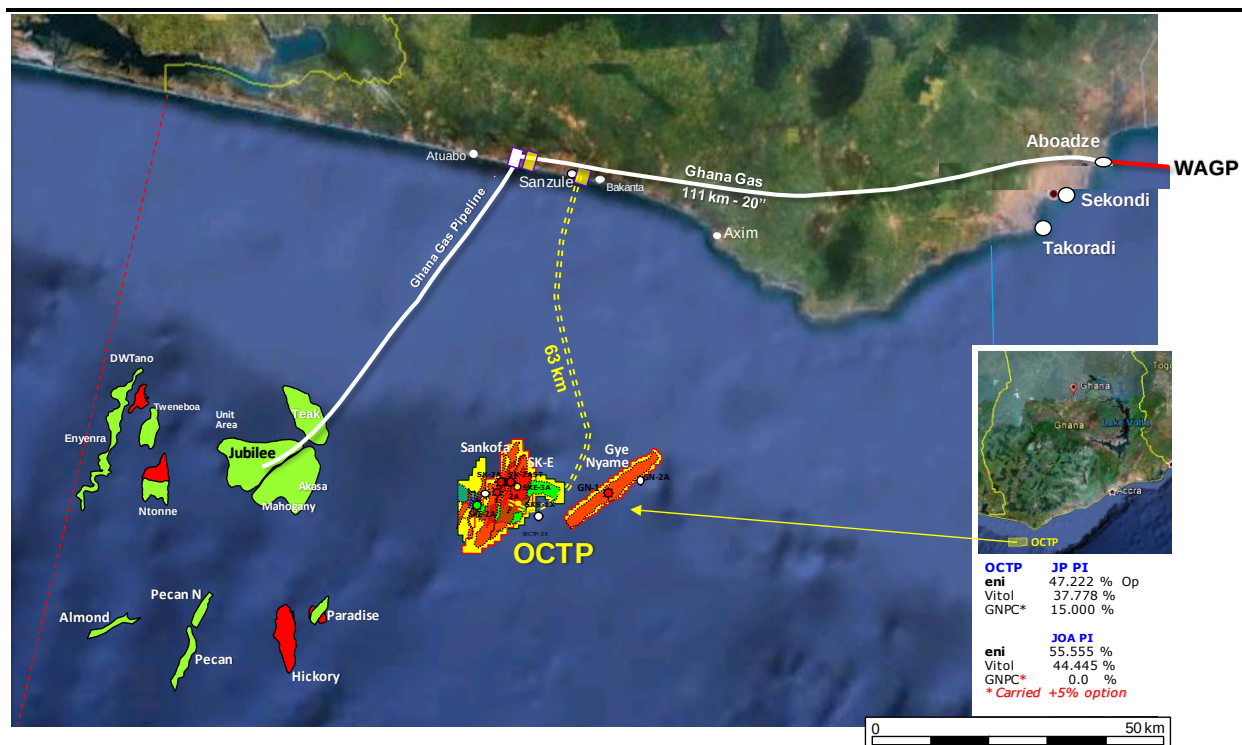
Figure 4.2 Project Location (Phase 2 elements in yellow)
