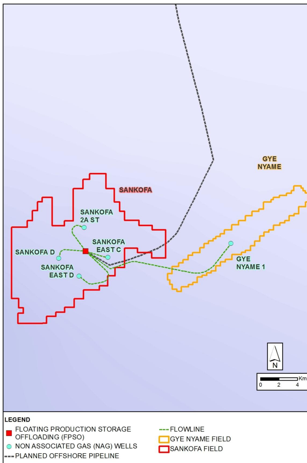
Figure 4.6 NAG Well Locations
