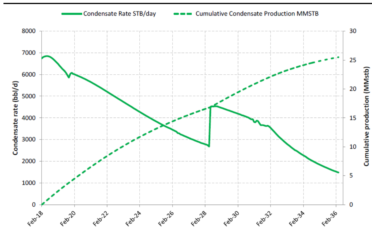
Figure 4.4 Profile of Condensates Production
