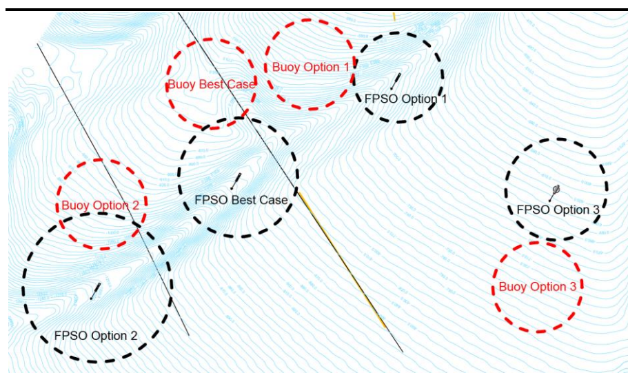
Figure 4.34 FPSO Location Options
