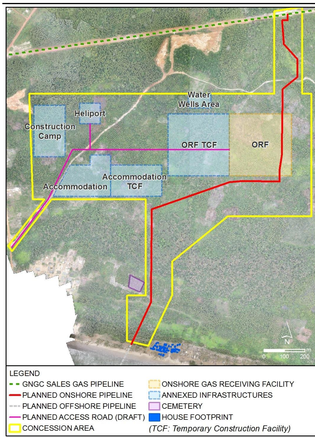
Figure 4.17 Gas Export Pipeline Landfall Location under Investigation
