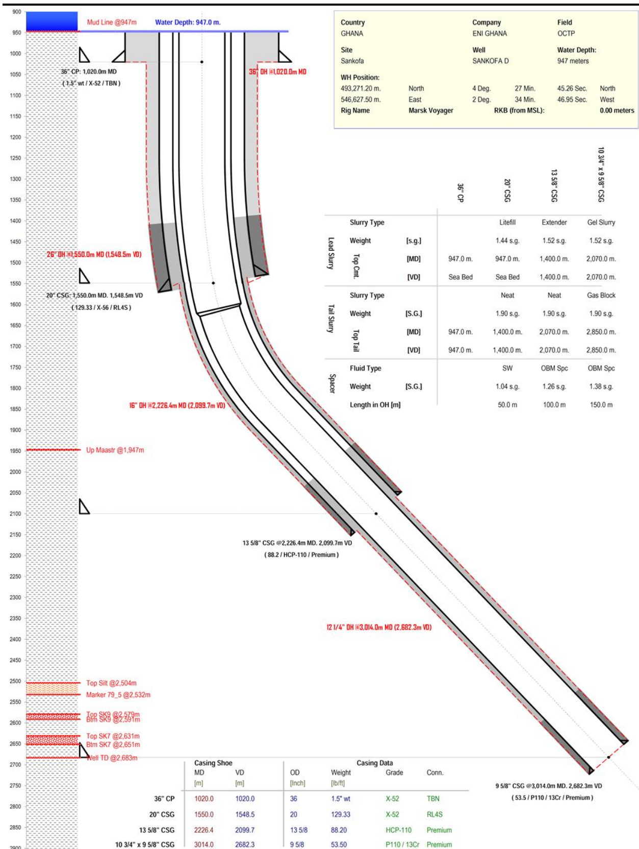
Figure 4.22 Typical Casing Profile
