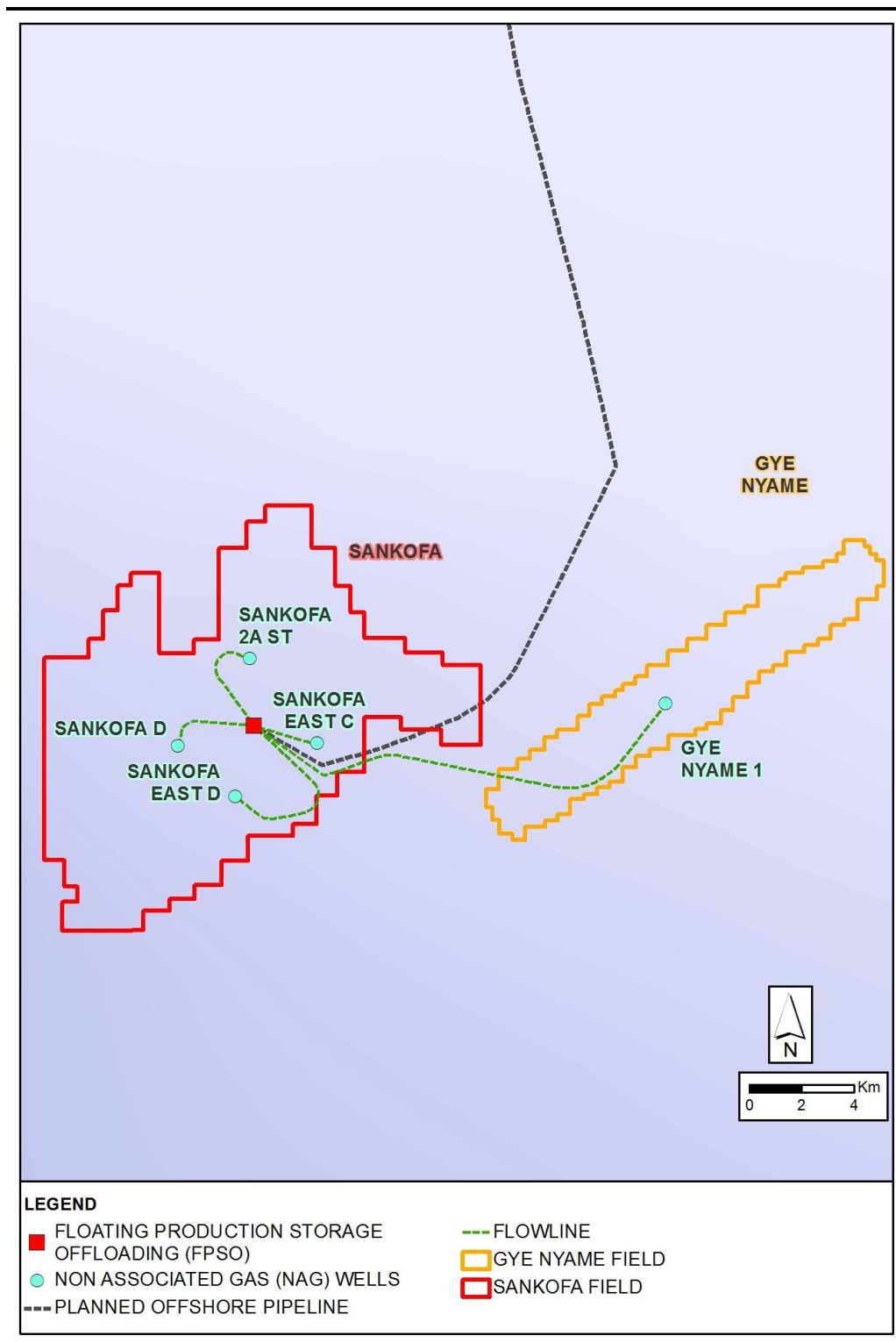
Figure 1.3 NAG wells and flowlines layout
