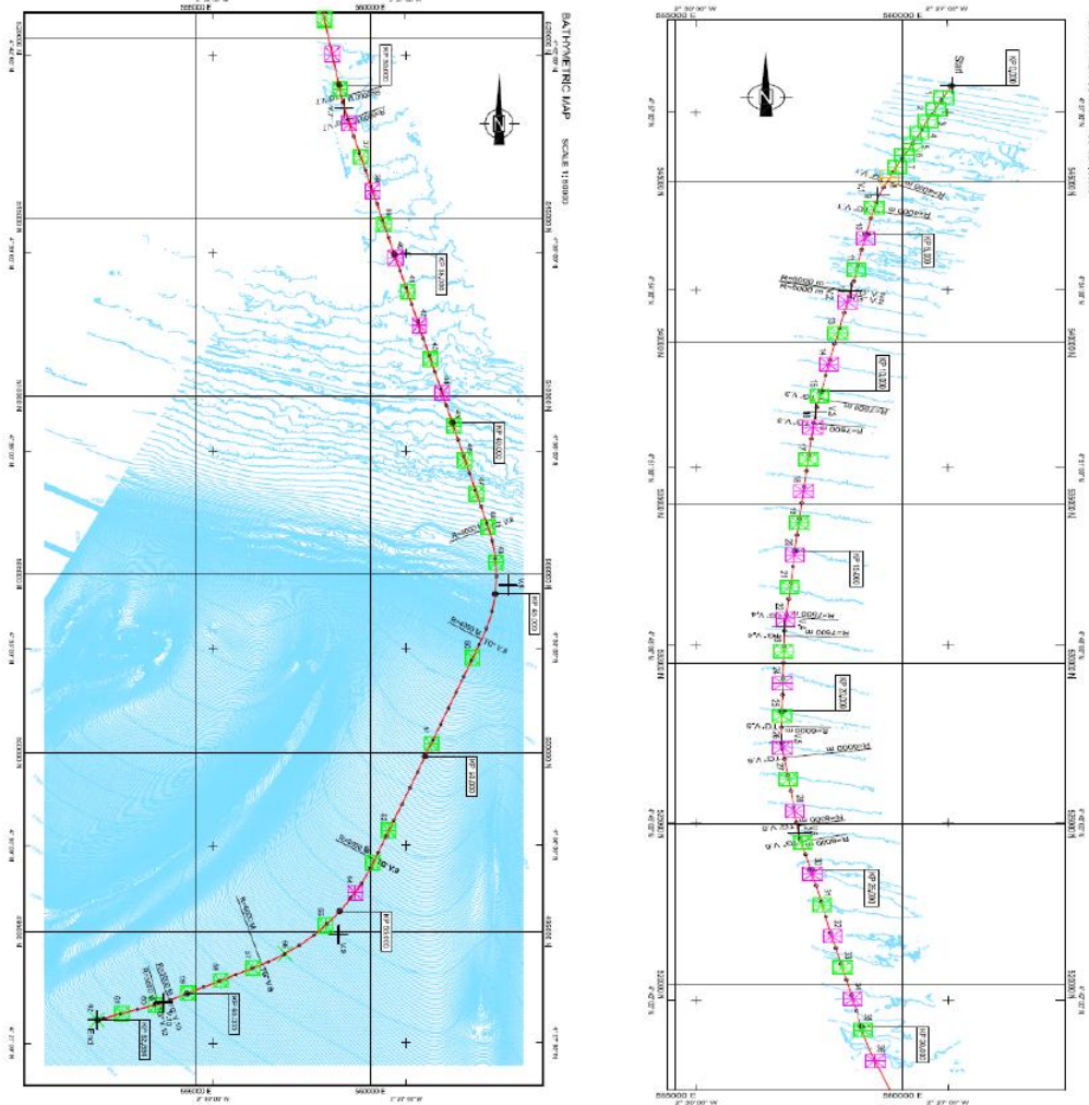
Figure 4.16 Export Gas Pipeline Route Left: Deepwater. Right: shallow Water.
