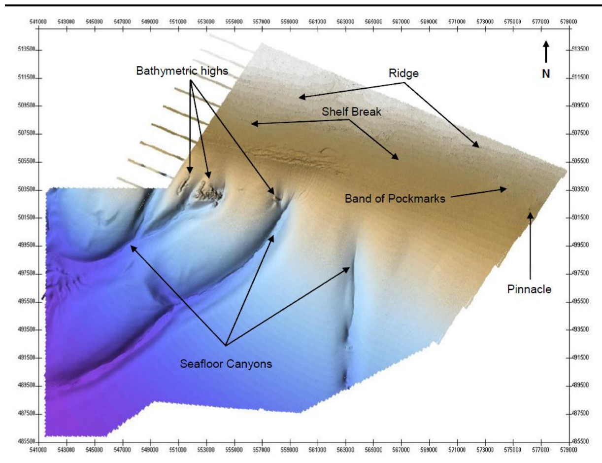
Figure 6.14 Bathymetry in the Project Area
