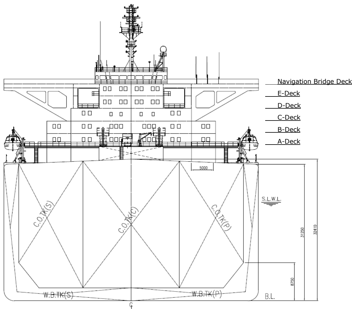
Figure 4.10 FPSO Typical Living Quarters view
