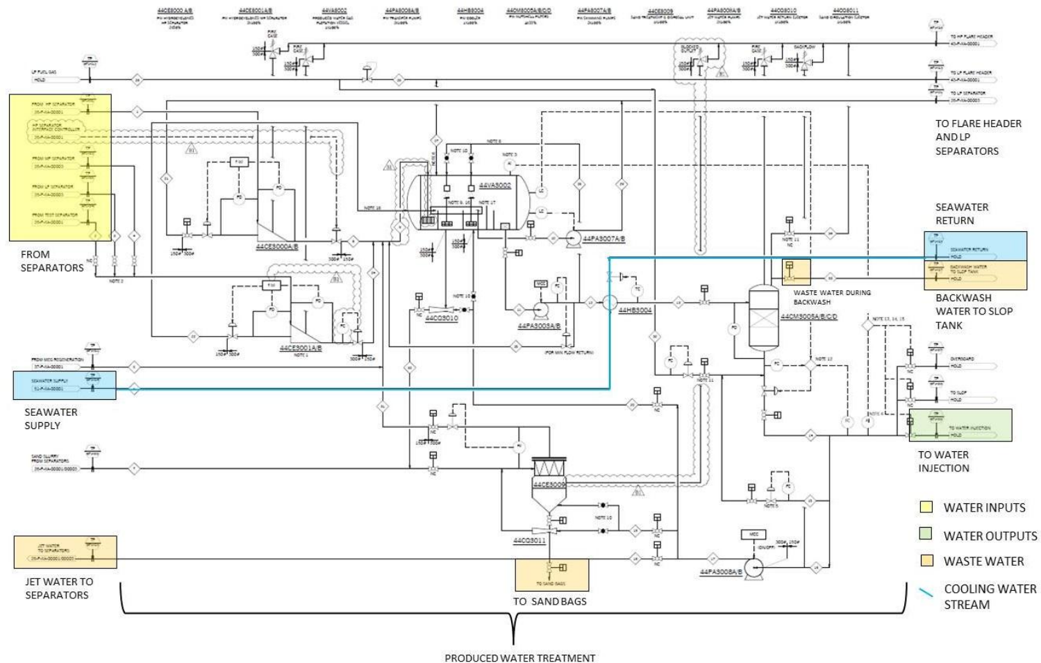
Figure 4.12 Produced Water Treatment Flow Diagram
