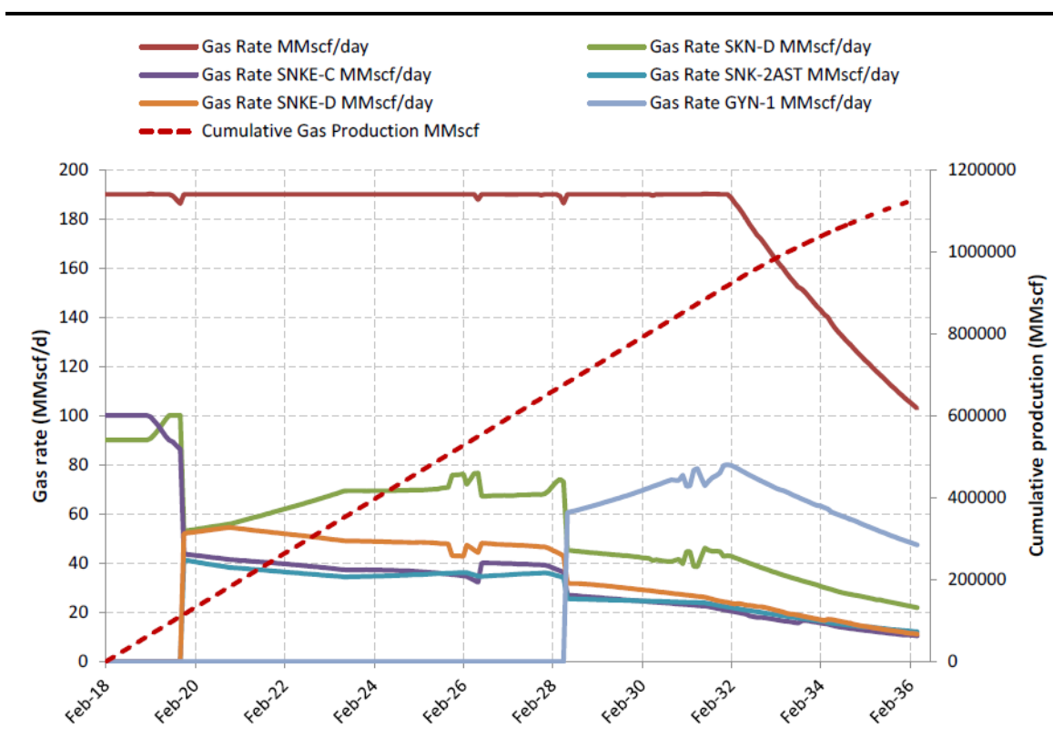
Figure 4.3 Profile of Raw Gas Production
