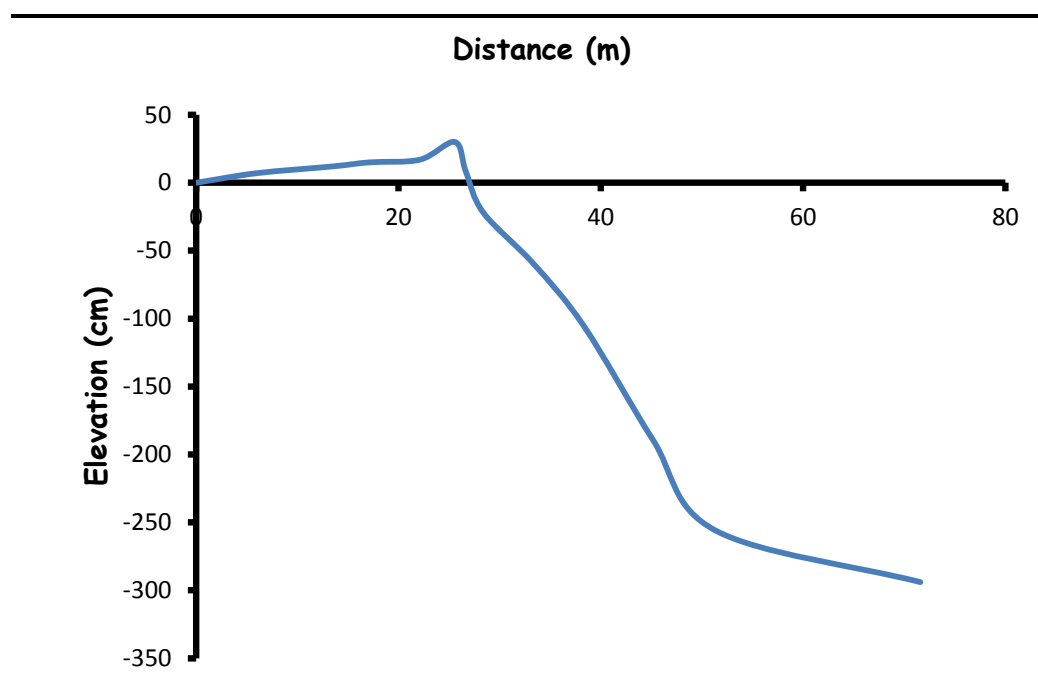
Figure 6.20 Beach profile at pipeline landfall site
