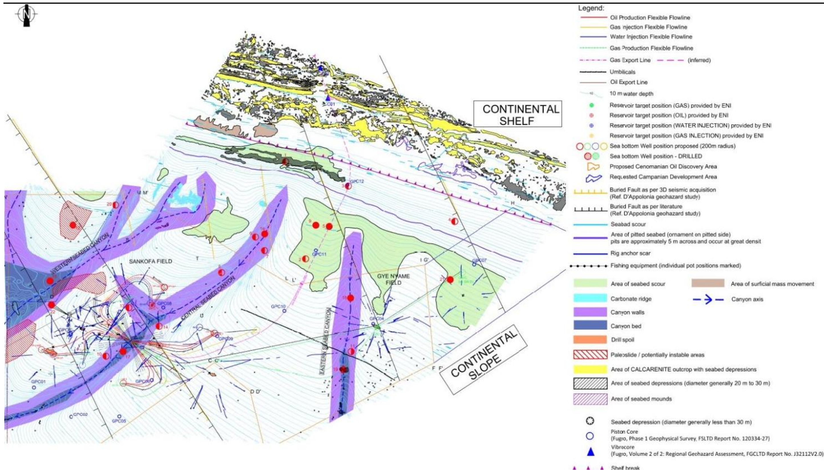
Figure 6.16 Subsea Geohazards in the Project area
