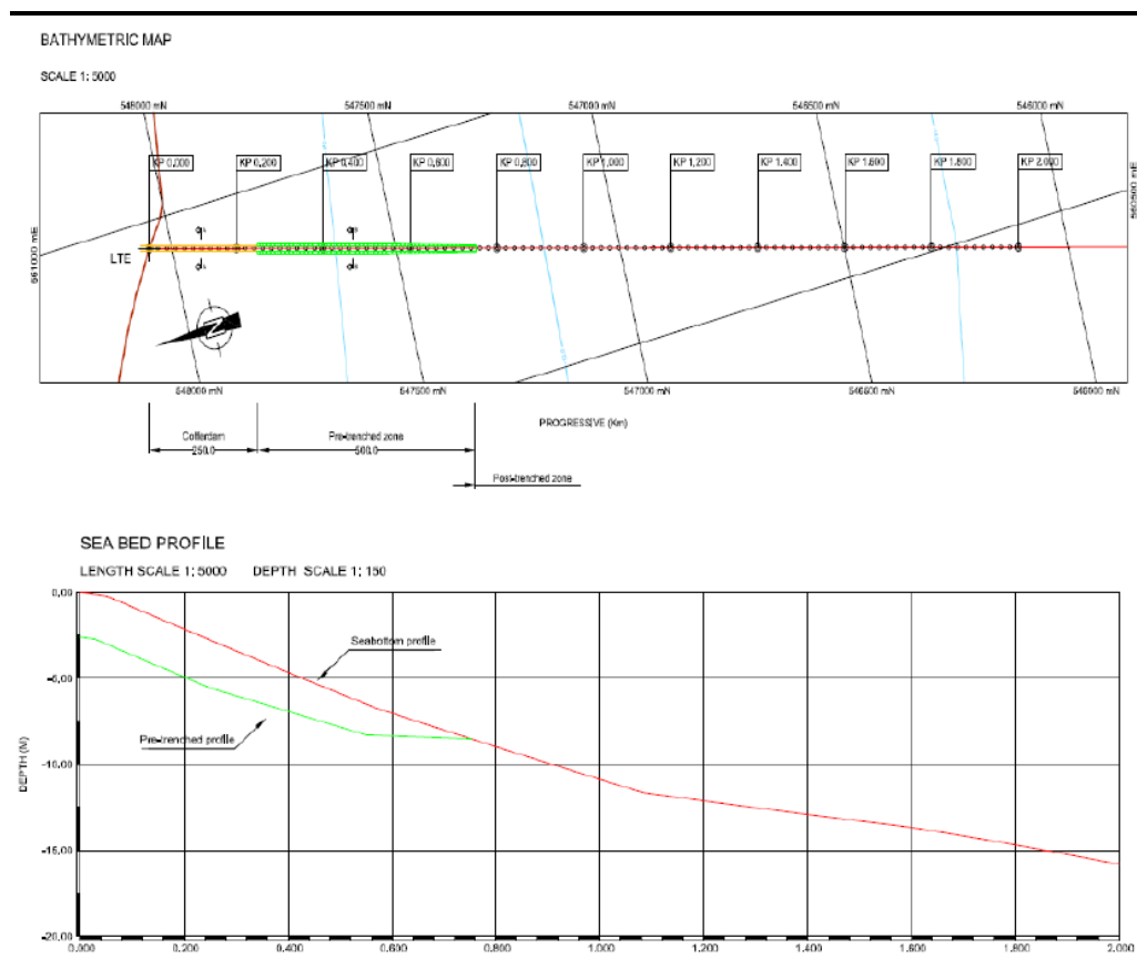
Figure 4.18 Preliminary Gas Export Pipeline Landfall Approach
