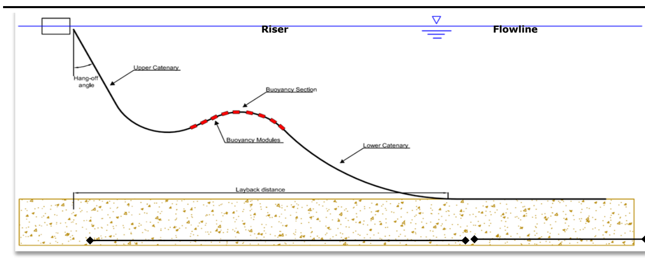
Figure 4.7 Lazy Wave Configuration
