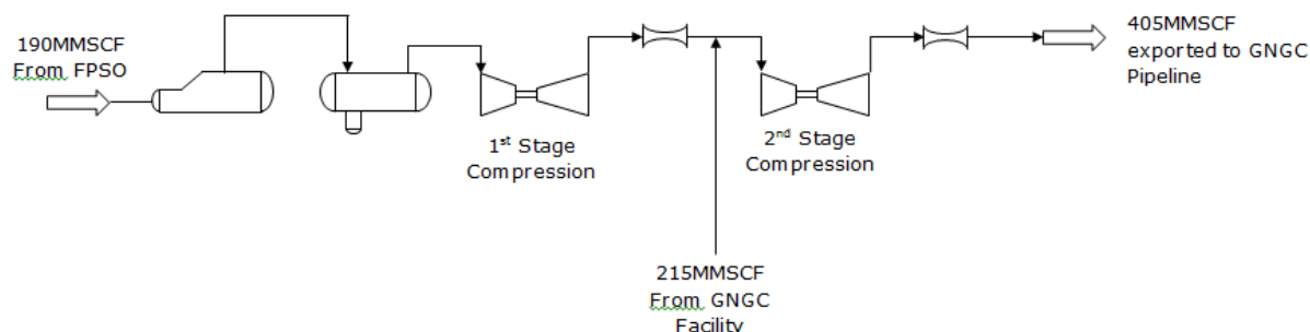
Figure 4.5 ORF flow diagram
