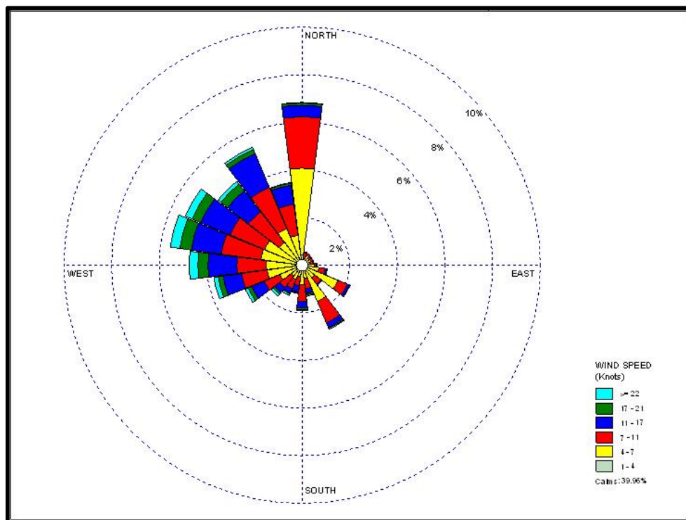
Figure 32: Wind speed and direction in Ma'an weather station for the Year (2004-2010)
