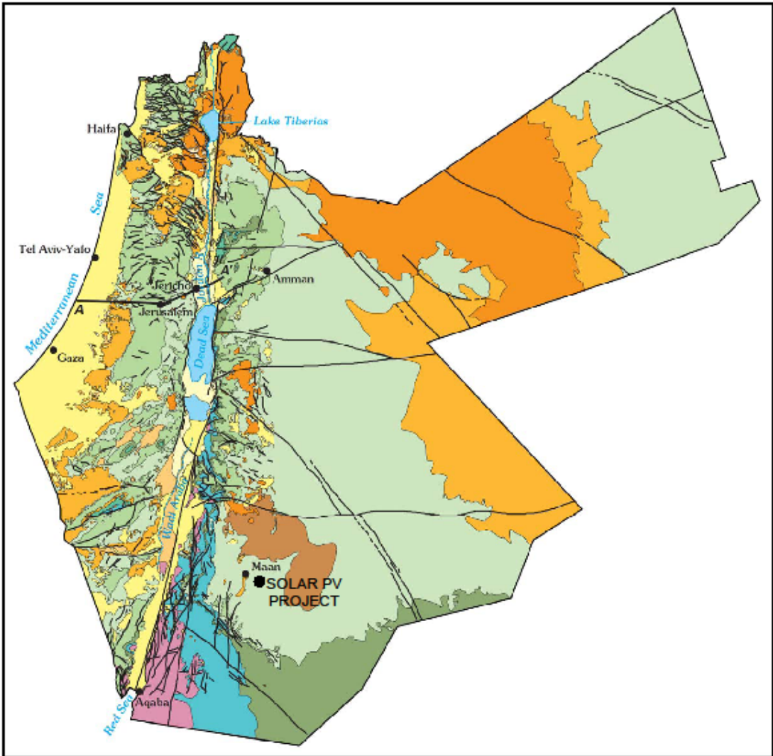
Figure 14: The Geology of Jordan
