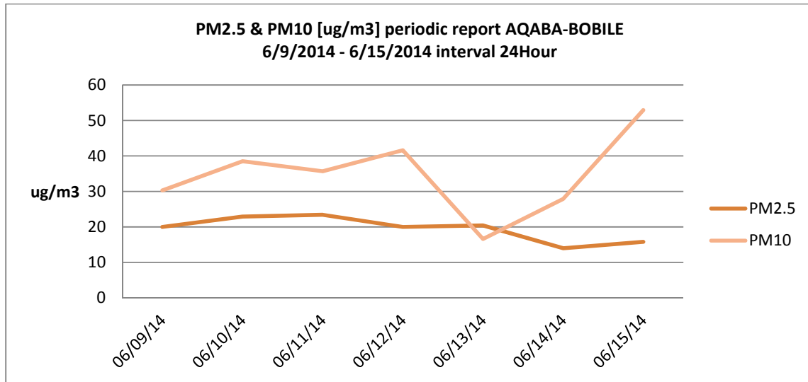
Figure 43:PM 2.5 & Pm 10 Concentration- 24 hours at the project site.
