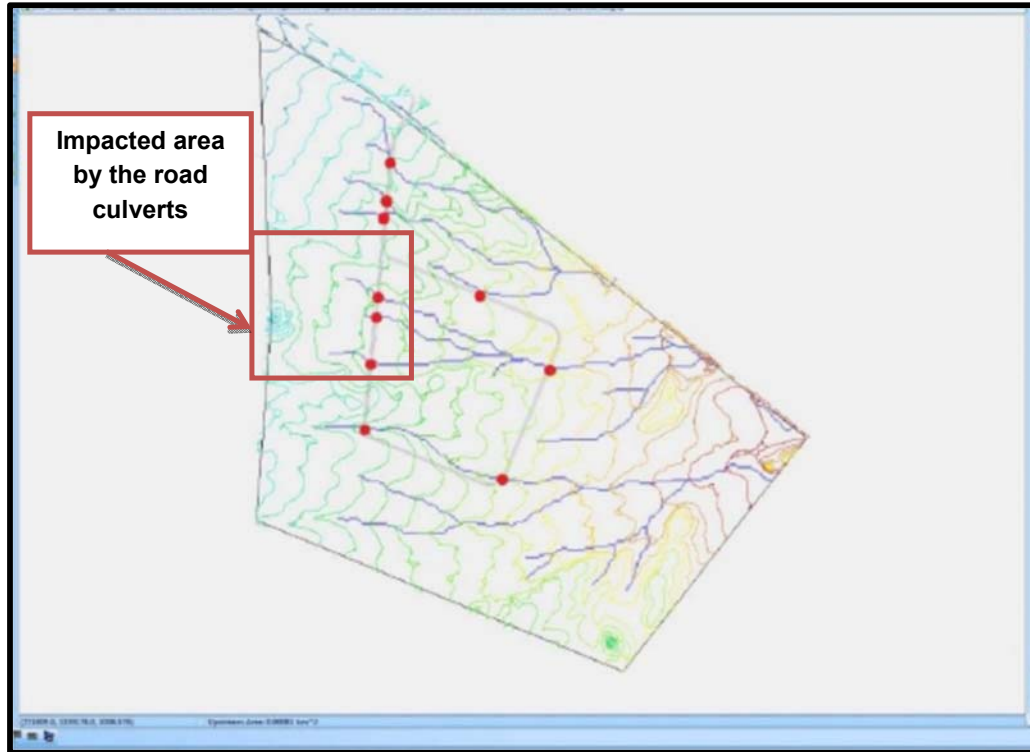
Figure 66: WMS Simulation for Wadi and Road intersection Points
