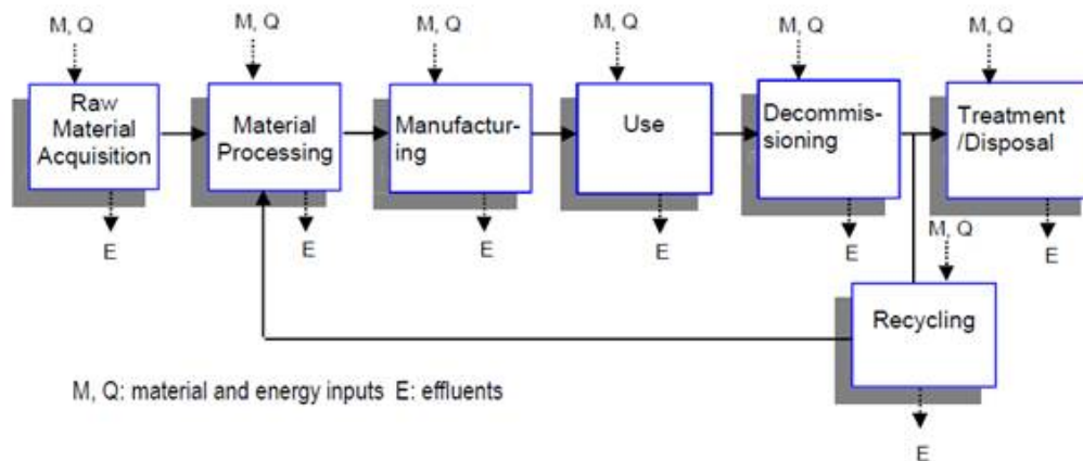
Figure 57:Material and energy inputs / outputs during the PV project lifecycle from cradle to grave (or cradle) (IEA.2011)
