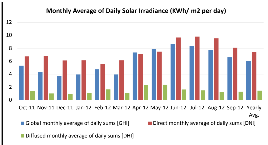
Figure 33: Monthly Average ( December)of Daily Solar Irradiance Sums ( kWh/m 2 perday)
