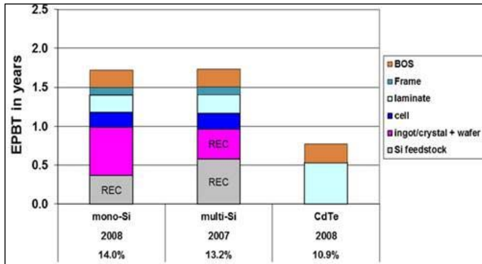
Figure 62: Energy payback time (EPBT) for PV technologies (Source: IEA,2011)
