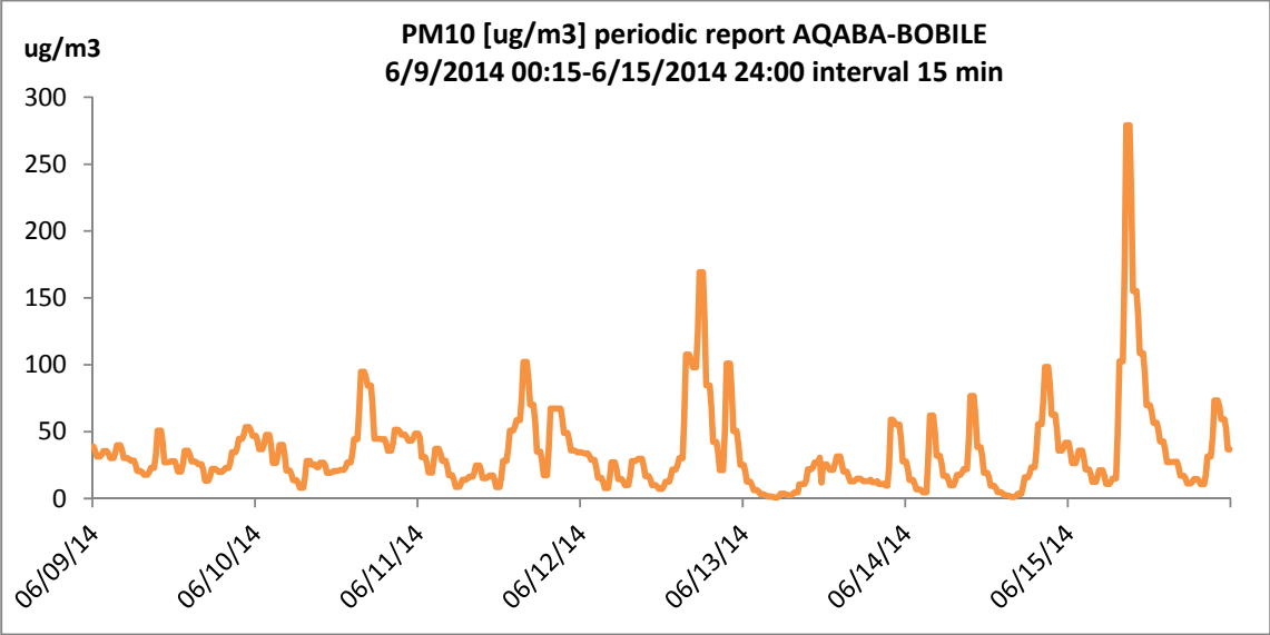
Figure 35:PM10 Concentration- 15 min average at theproject site.
