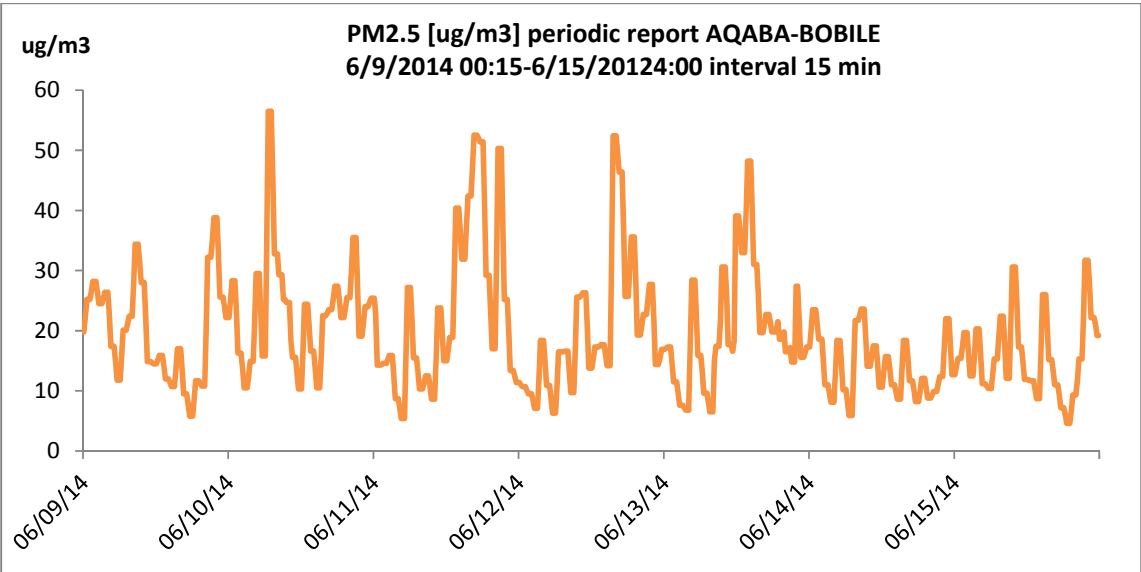
Figure 38:PM 2.5 Concentration- 15 min average at the project site.
