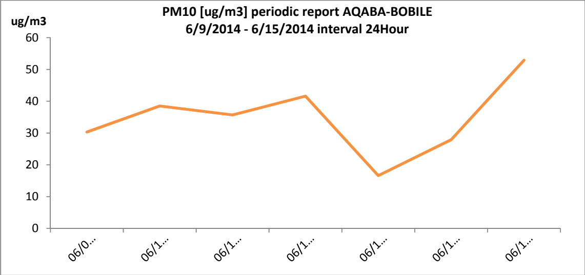
Figure 37:PM10 Concentration- 24 hours at the project site.
