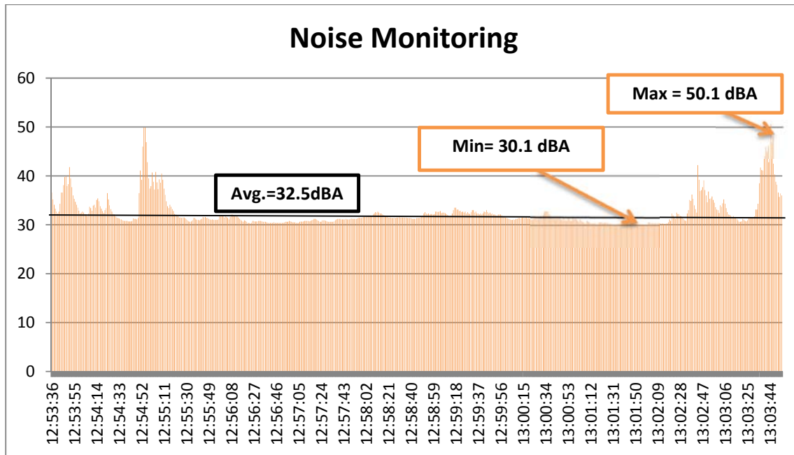
Figure 45: Results of Noise Monitoring
