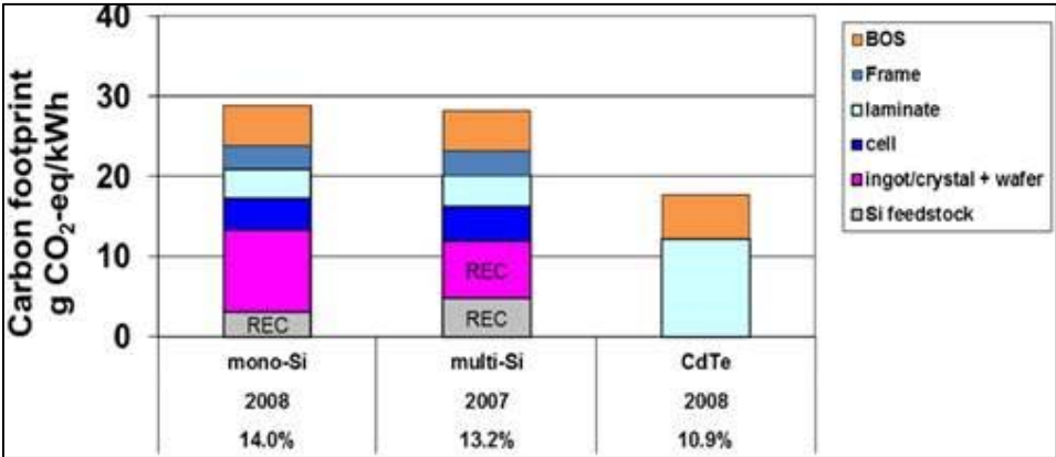
Figure 60: Carbon foot print of crystalline and thin-film roof mounted PV systems (IEA, 2011)
