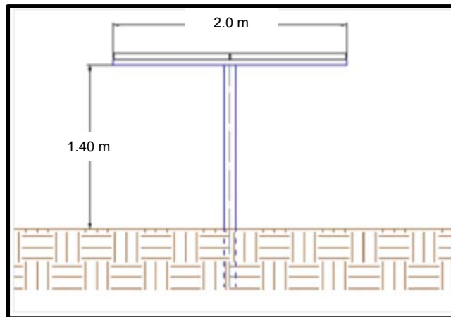
Figure 5 : Structure details
