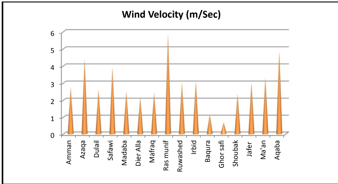
Figure 31: Average Wind Speed in Selected Locations in Jordan
