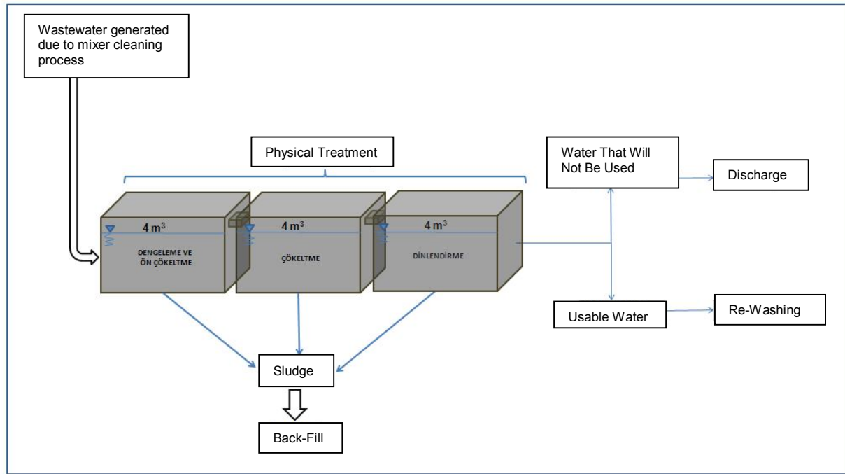
Figure 56. Settling Tank
