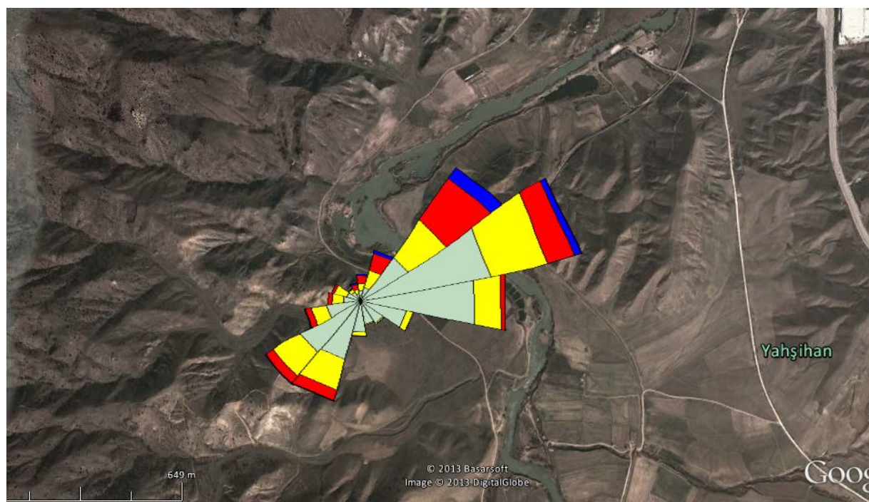
Figure 73. 2012 Wind Rose
