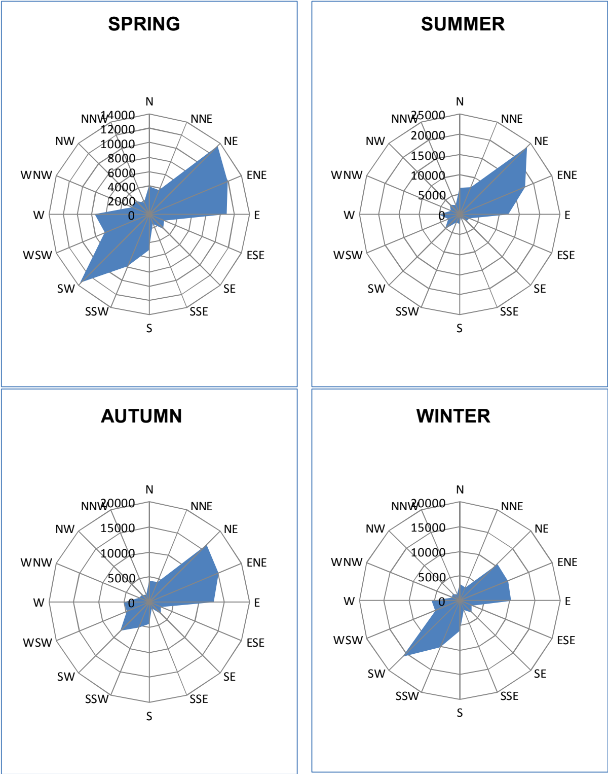
Figure 24. Kırıkkale Meteorology Station Blowing Numbers of Wind According to Seasons Graph
