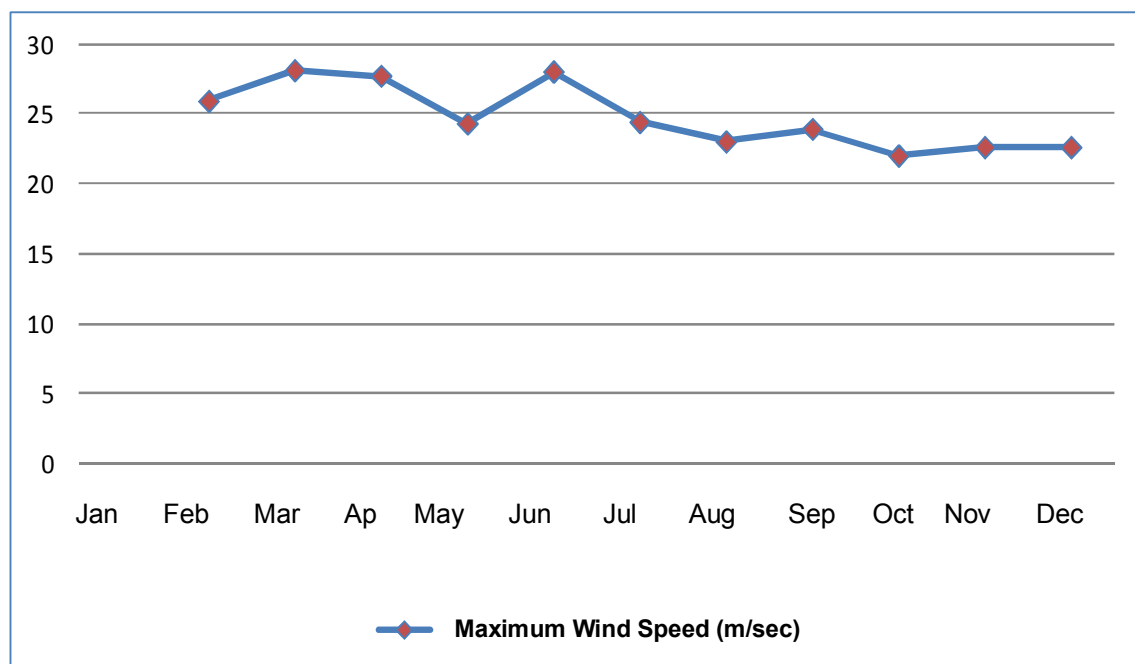
Figure 28. Kirkkale Meteorology Station Maximum Wind Speed Graph
