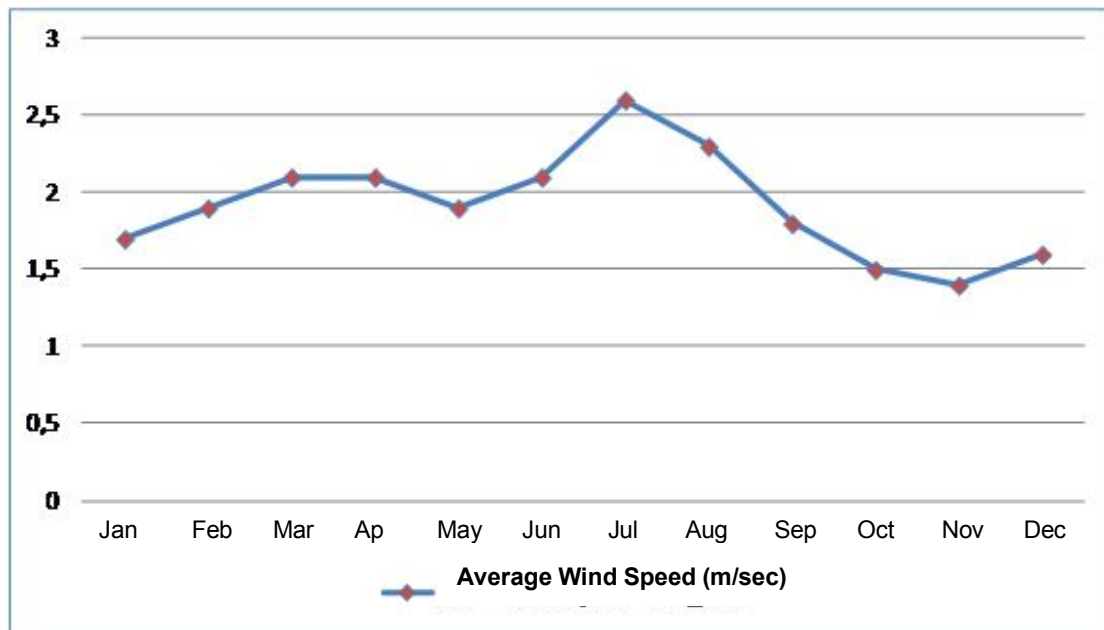
Figure 27. Kirkkale Meteorology Station Average Wind Speed Graph
