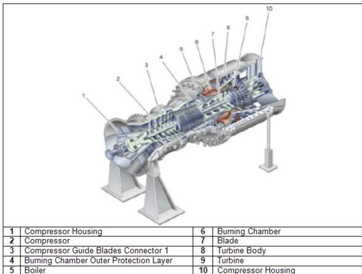
Figure 60. General Cross Section of Cylindrical Burning Chamber and Gas Turbine
