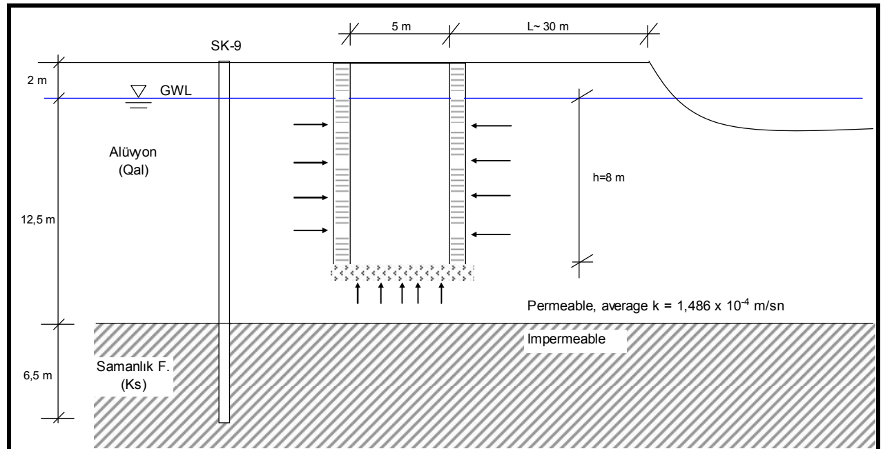
Figure 37. Approximate dimensions and position of a well, which could be excavated near to borehole SK-9.
