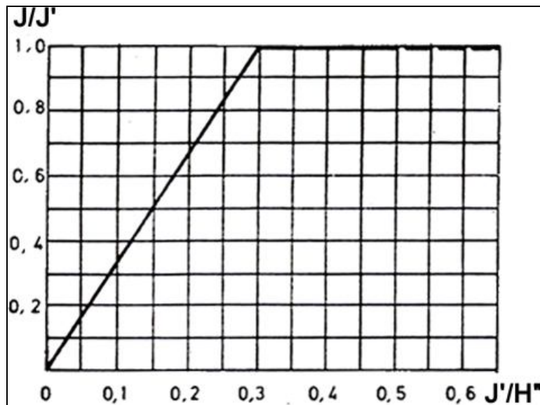
Figure 82. Abac to be used for Calculation of J/J' Value
