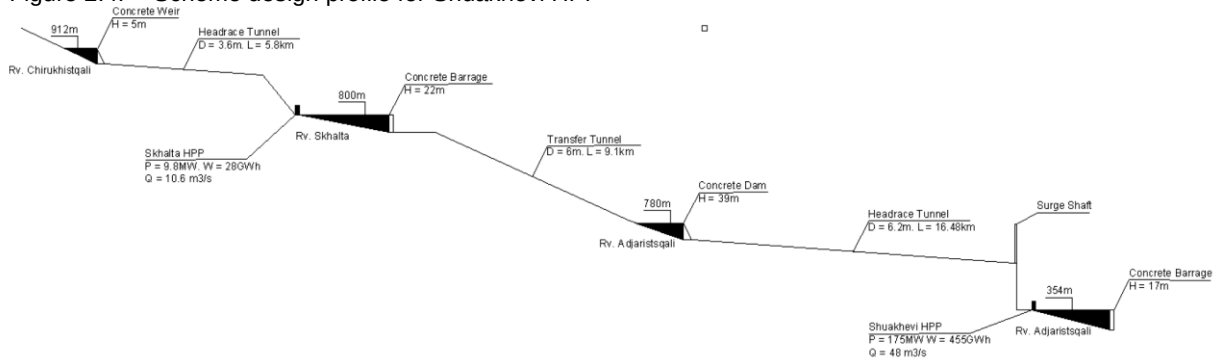
Figure 2.4: Scheme design profile for Shuakhevi HPP
