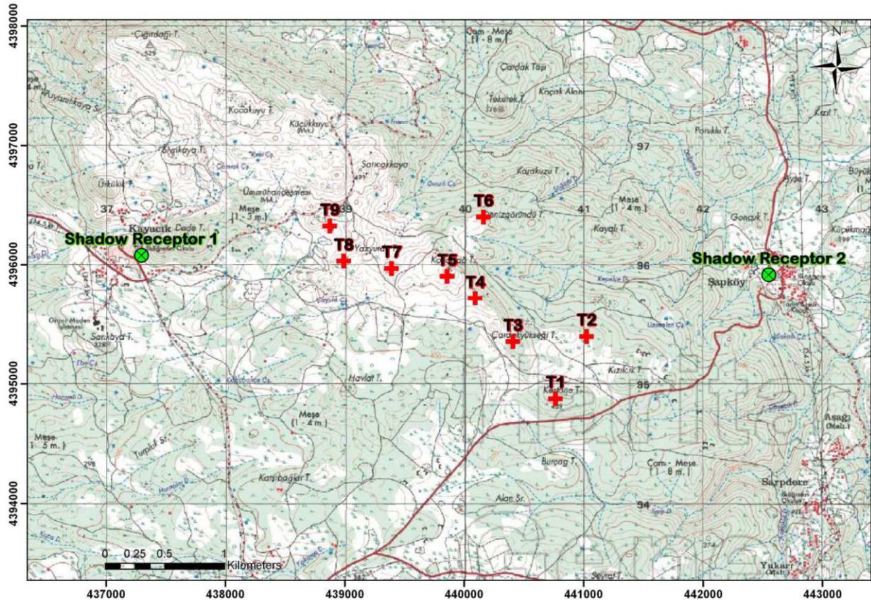
Figure 5-9 Locations of Shadow Receptors
