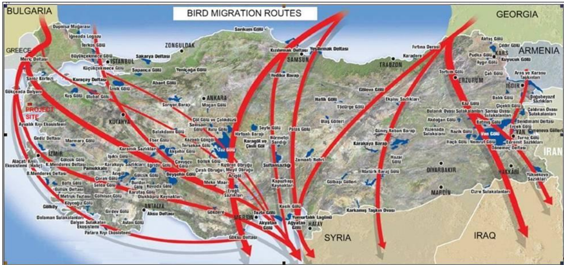
Figure 4-27 Bird Migration Routes in Turkey
