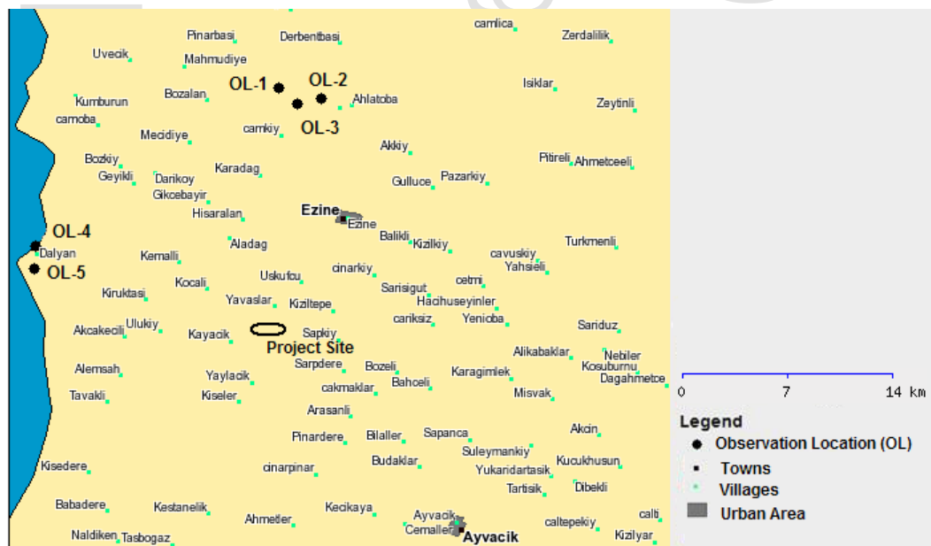
Figure 4-26 Closest Observation Locations to the Project Site in the Kuşbank Database
