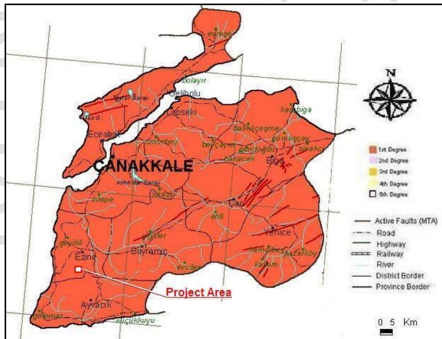
Figure 4-18 Earthquake Zone Map of Çanakkale Province
