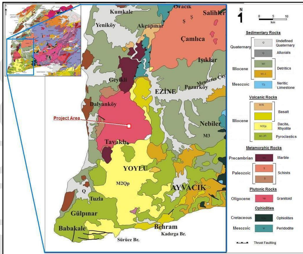
Figure 4-15 Regional Geological Map of the Biga Peninsula
