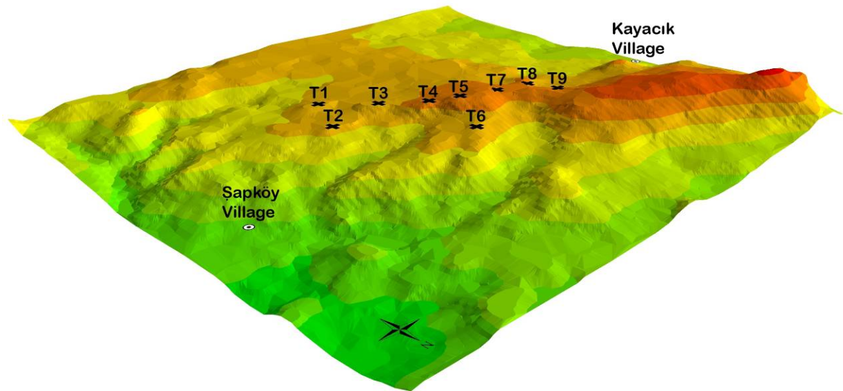
Figure 3-9 Three Dimensional Topography Map Looking Southwest
