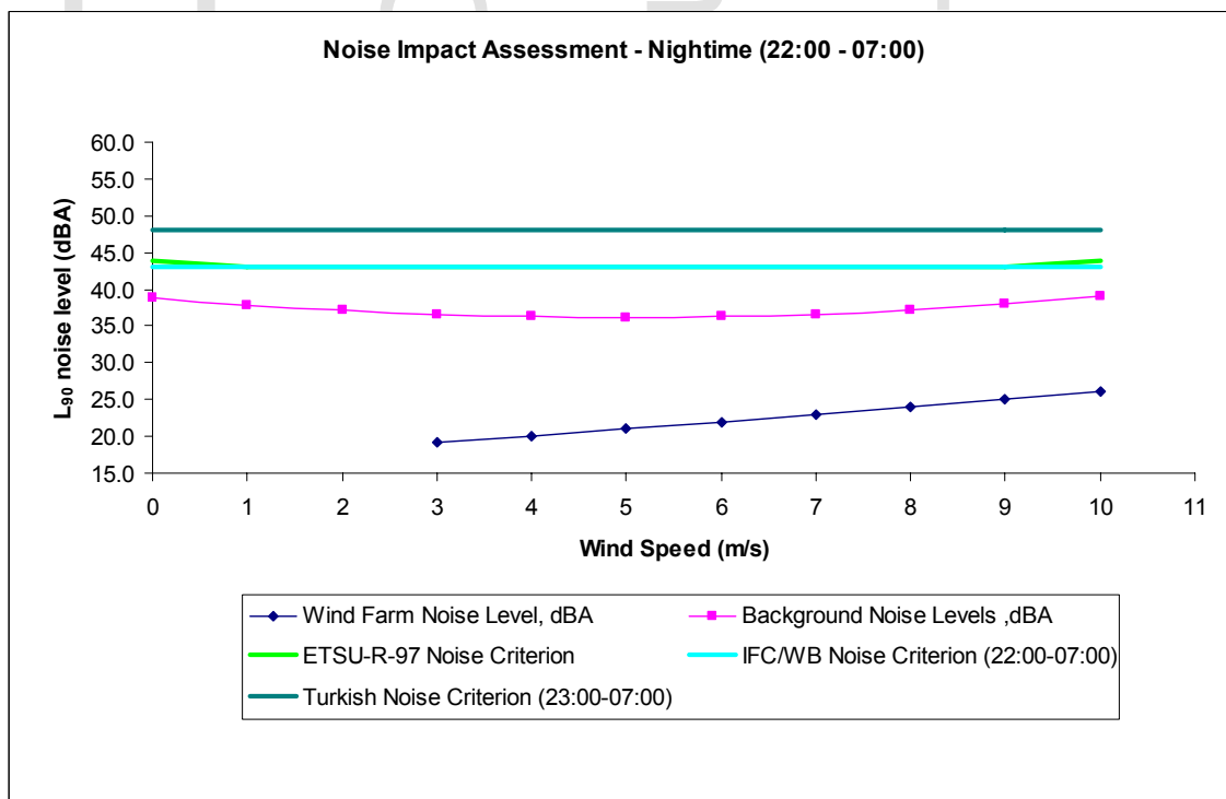
Figure 5-4 Daytime and Nighttime Wind Farm Noise Levels Compared to Noise Criteria
