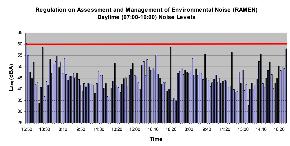
Figure 4-10 Daytime Background Noise Measurement Results compared to Turkish RAMEN
