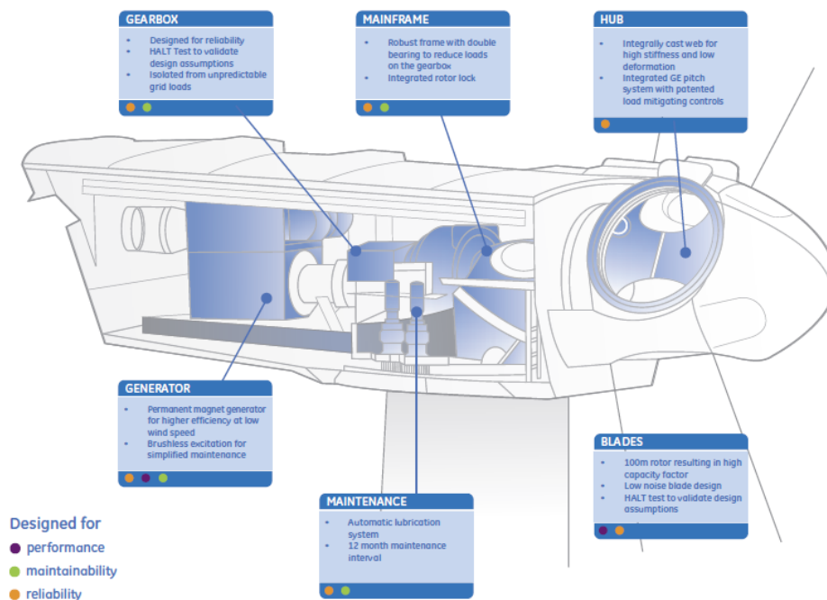
Figure 3-11 View of Nacelle
