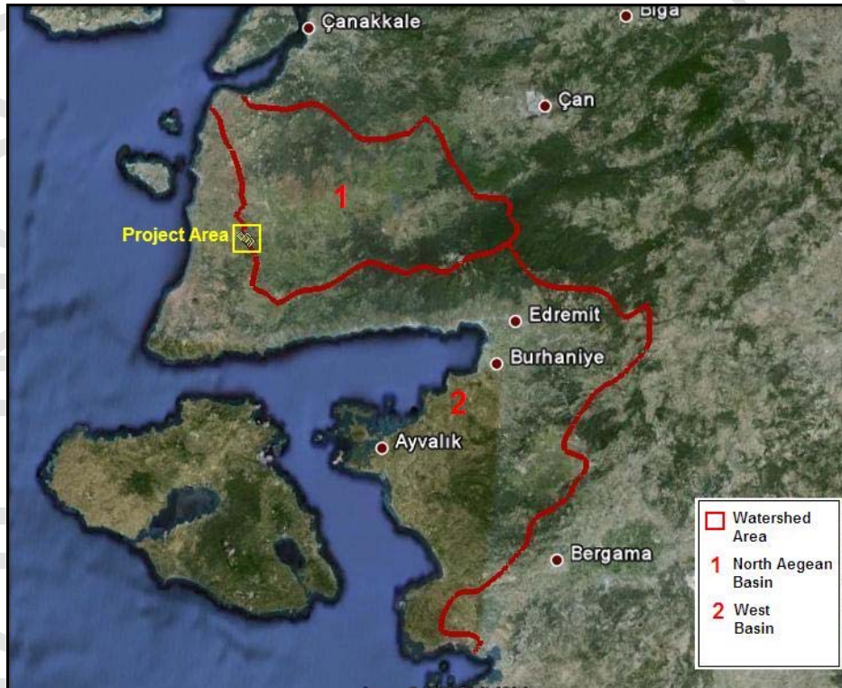
Figure 4-21 Basins in the Region (Source: Modified from Google Earth, 2009)
