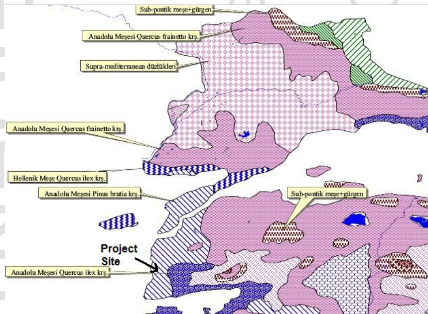
Figure 4-24 Natural Vegetation Map
