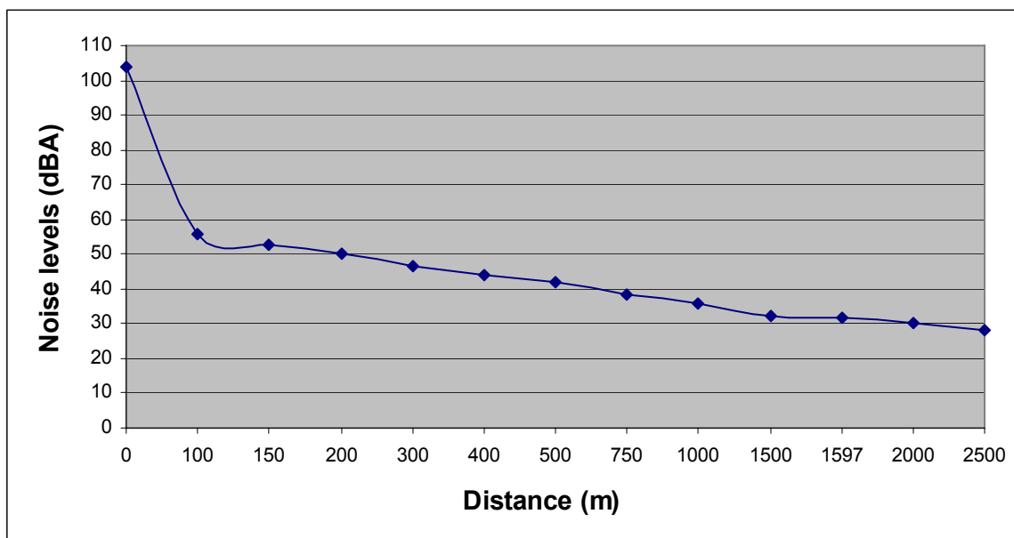
Figure 5-1 Noise Distribution during Construction
