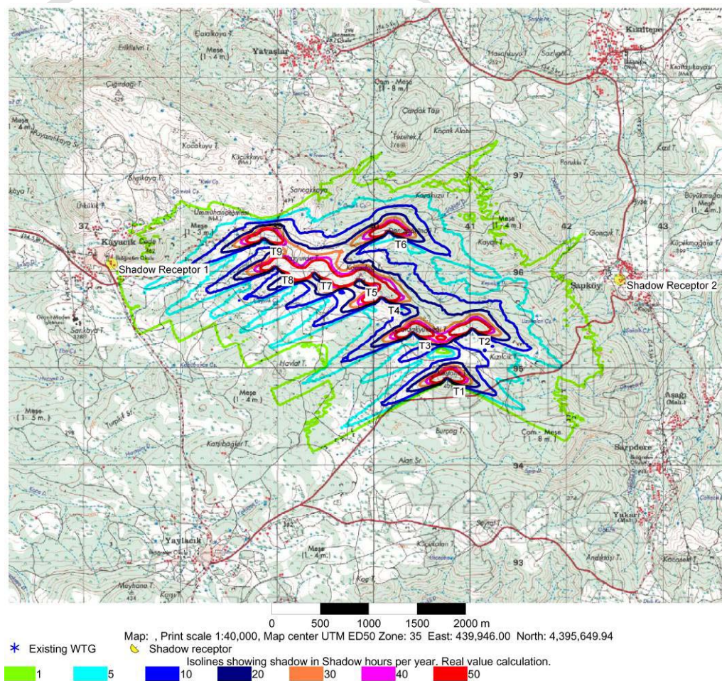
Figure 5-10 Realistic Case Shadow Contour Map
