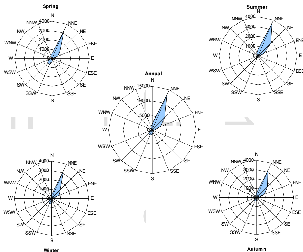
Figure 4-2 Annual and Seasonal Wind Roses
