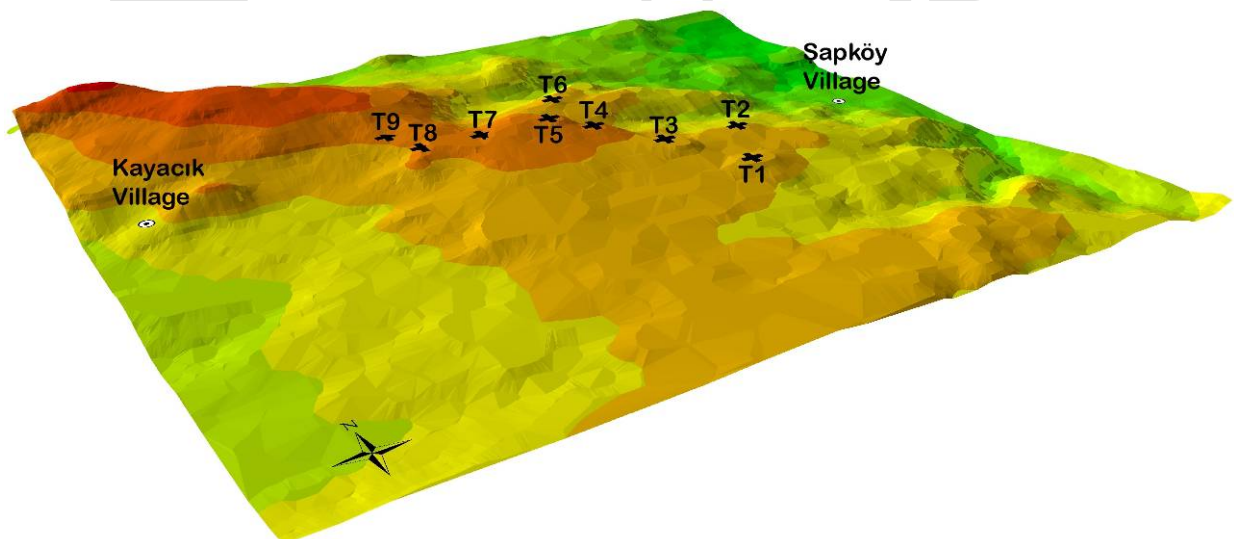
Figure 3-8 Three Dimensional Topography Map Looking Northeast
