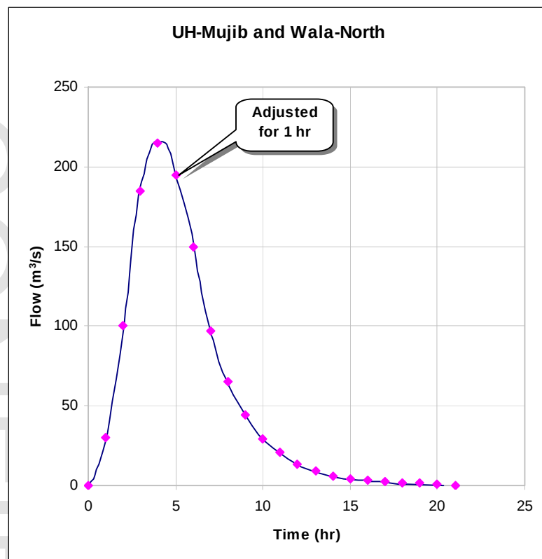
Figure 7: Unit-Hydrograph of Wadi Mujib and Wala-North
