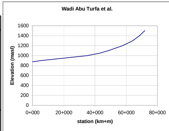
Figure 10: Stream Profile for Wadi Abu Turfa et al. with Slope Index Calculation
