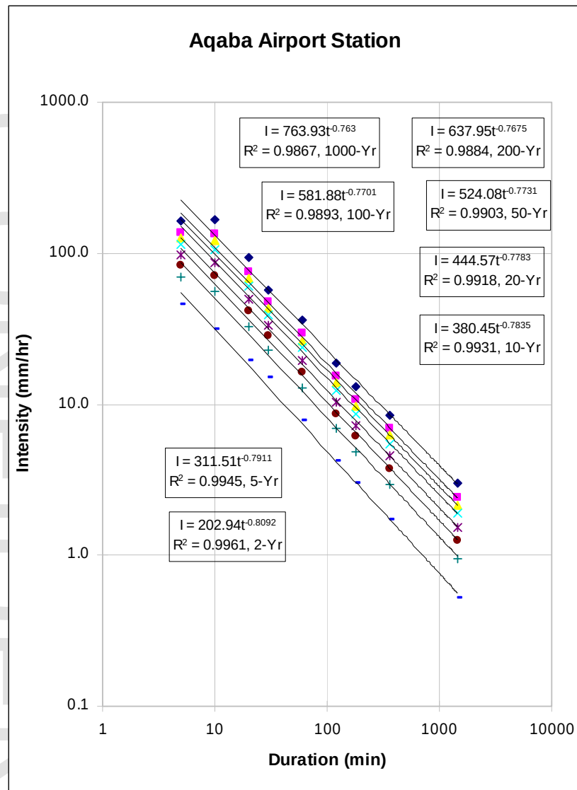
Figure 11: I-D-F Curves for Aqaba-Airport Rainfall Station
