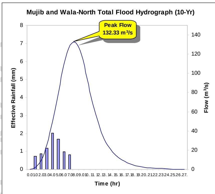
Figure 9: The flow Hydrograph for Wadi Mujib and Wala-North at 10-Yr return period with effective rainfall
