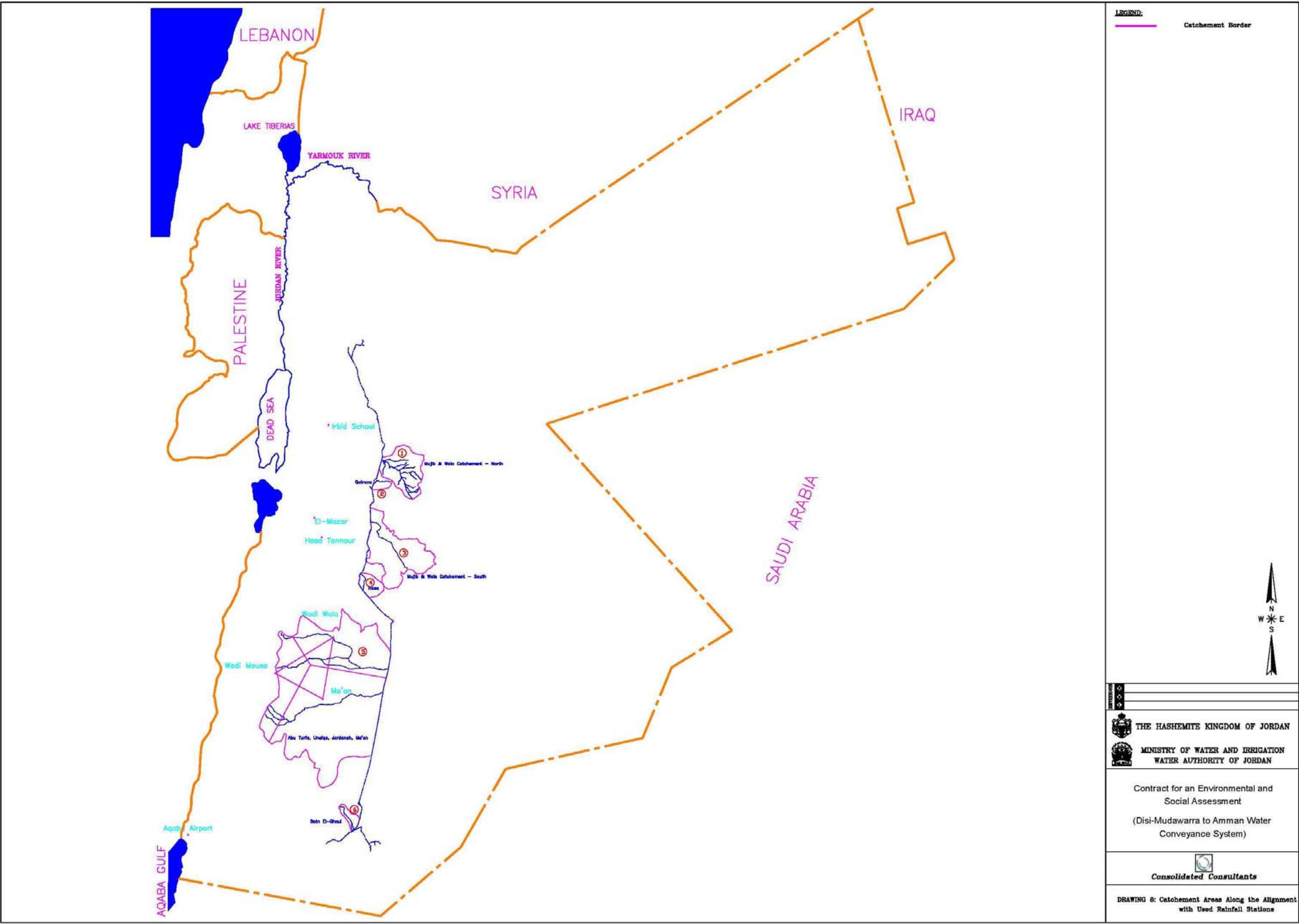
Drawing 8: Catchment areas along the alignment with used rainfall sections
