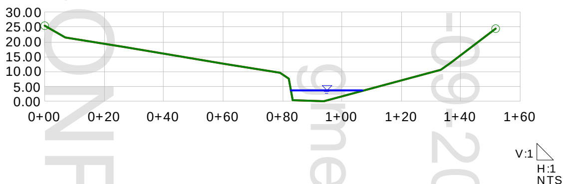
Figure 12: Wadi Abu Turfa Cross-Section 1
