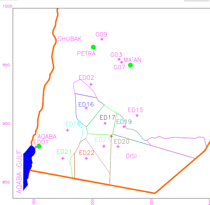
Figure 4: Thiessen Polygons for Disi Area
