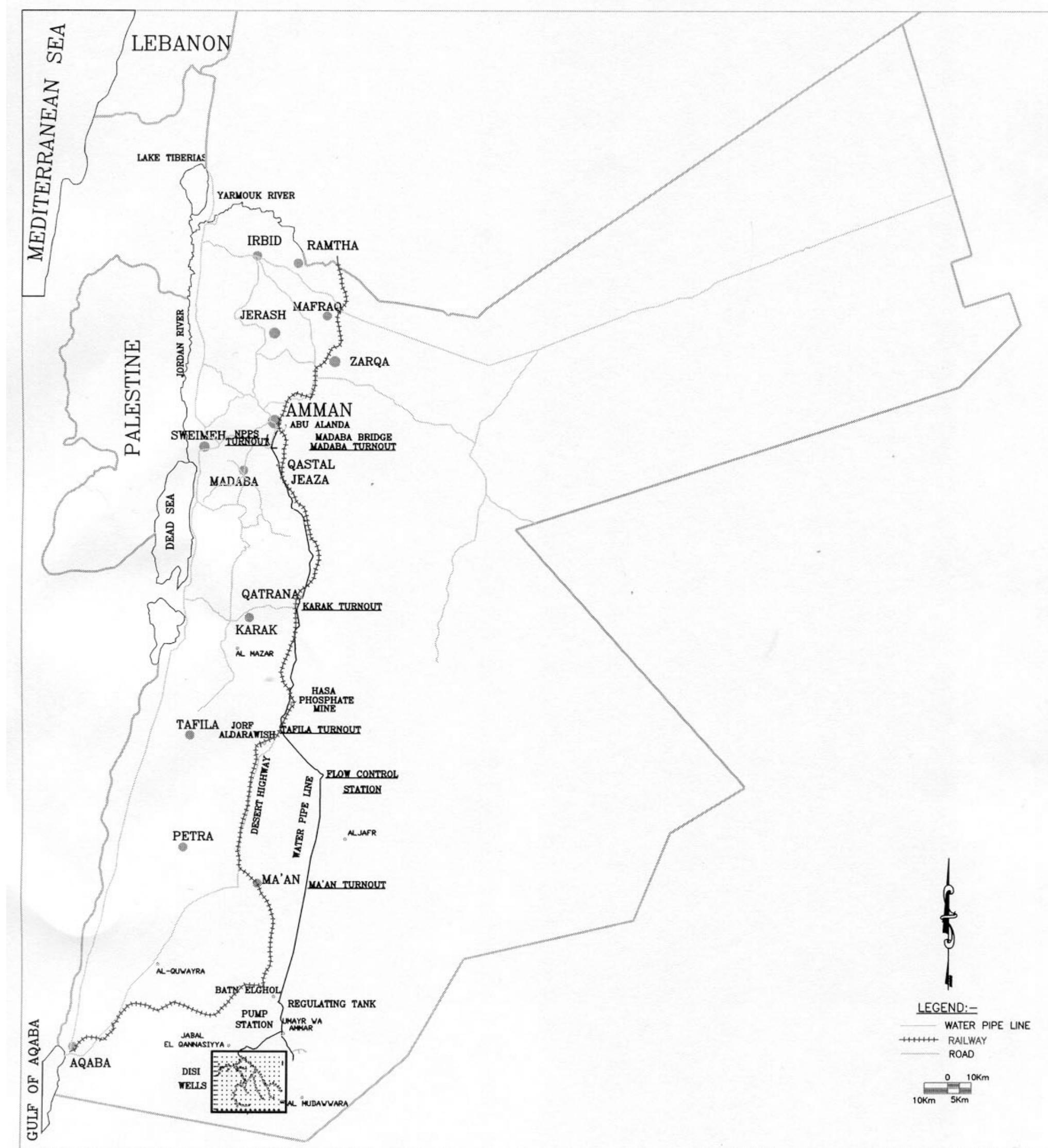
Figure 3: Optimised alignment of the Disi-Mudawarra to Amman water conveyance system
