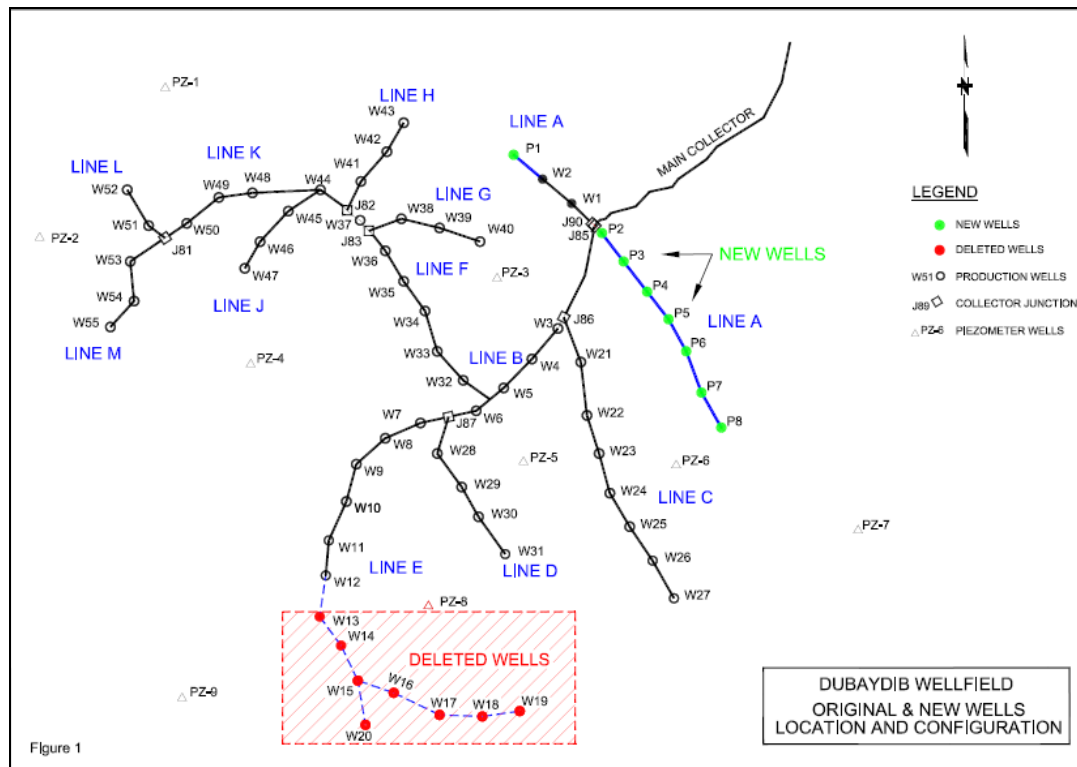
Figure 3.2 Revised Wellfield Layout
