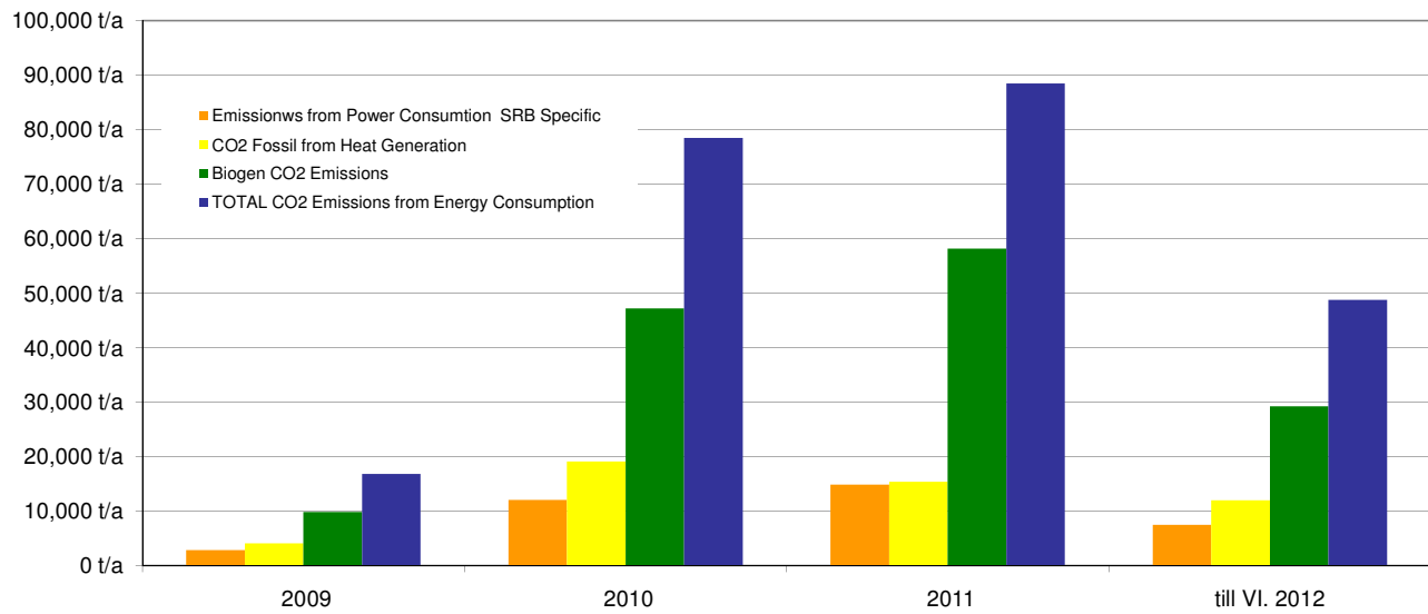
GHG - CO2 Emissions from Heat Generation and Power Consumption KRONOSPAN Lapovo 2009 till MDF project introduction VI. 2012
