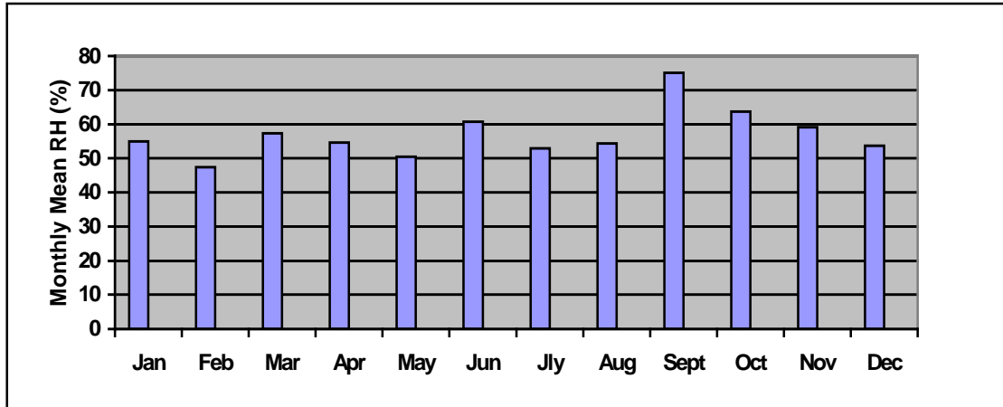
Fig 4.7 : Relative Humidity recorded at Fiche Observatory during 1986-2005
