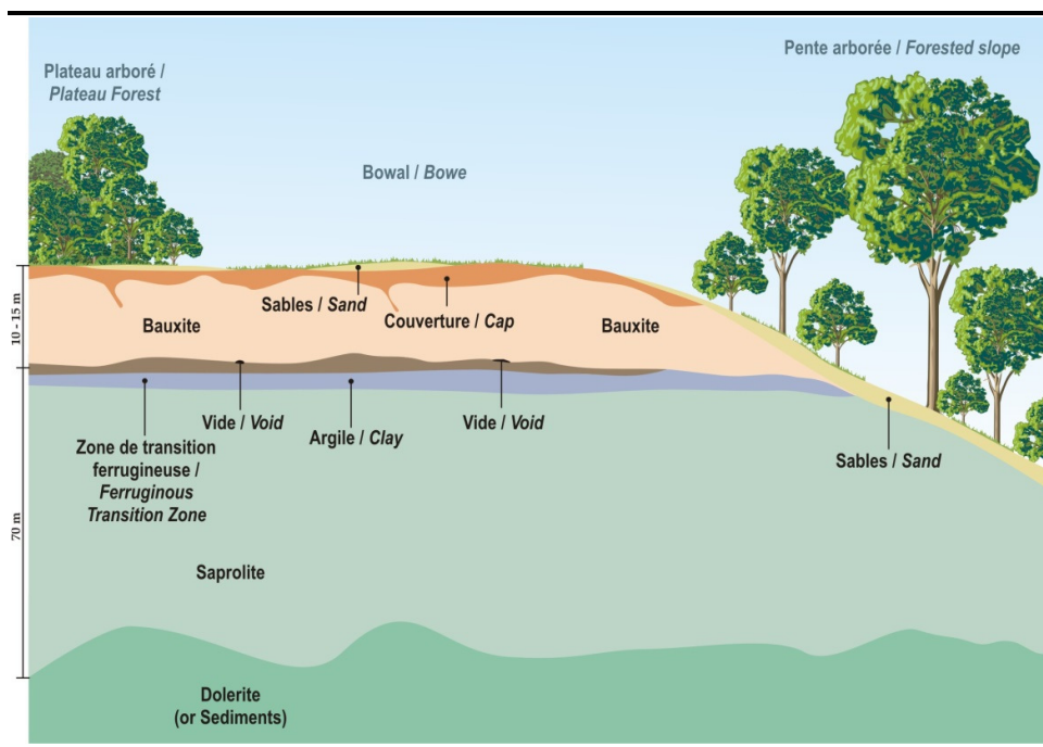
Figure 4.2 Illustrative geological cross-section of bauxite deposits in the GAC concession
