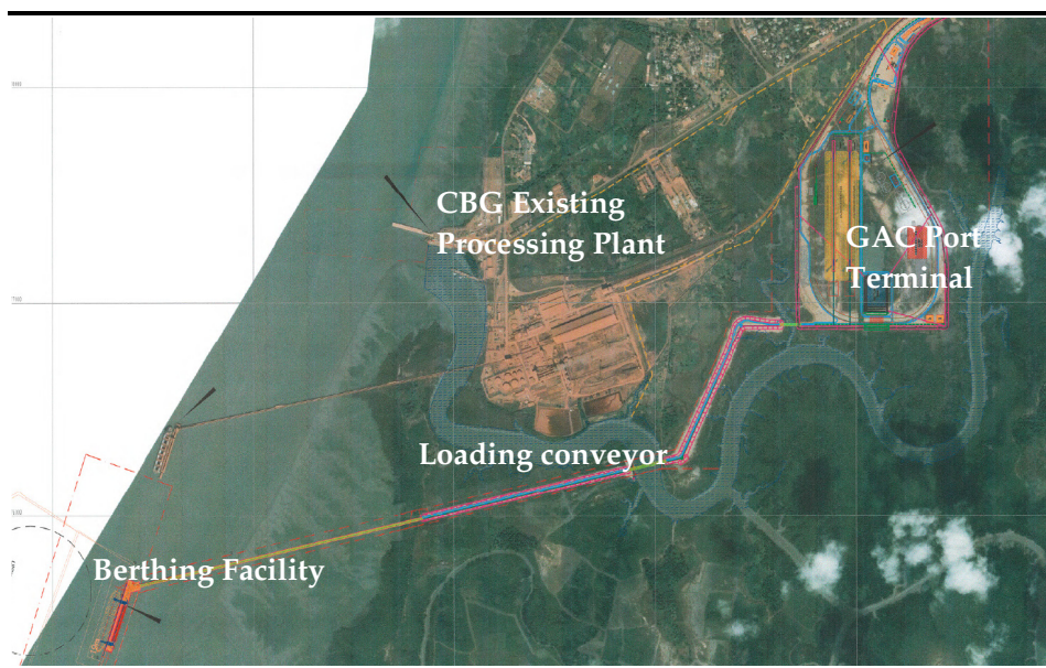
Figure 4.5 Overview of proposed port components
