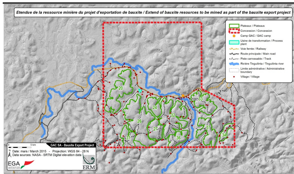
Figure 4.1 Extent of bauxite resources to be mined as part of the Project
