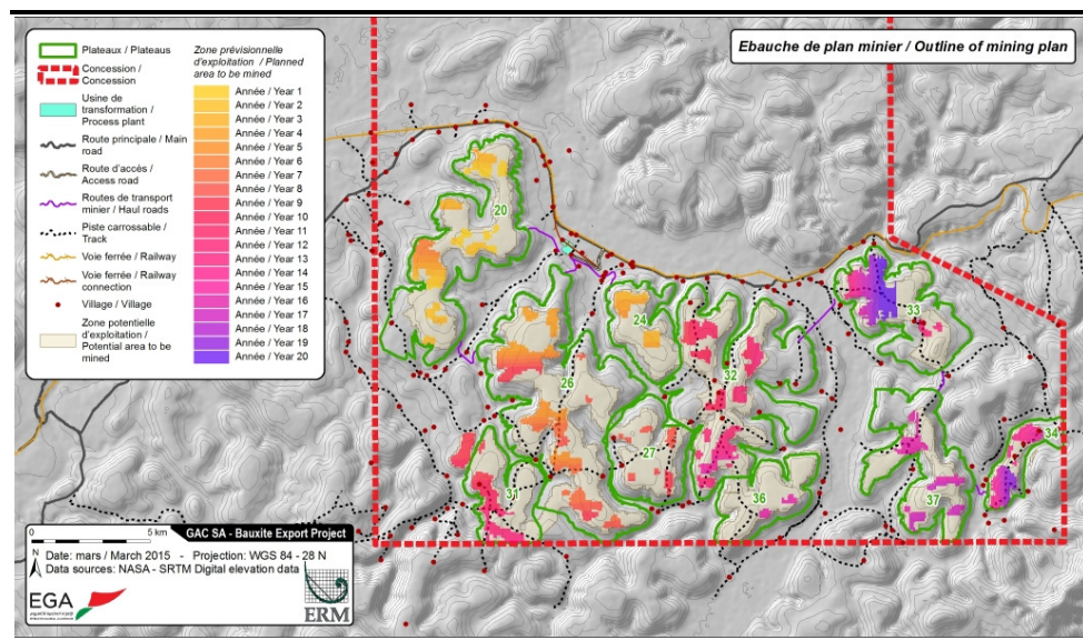
Figure 4.4 Outline of indicative mine plan
