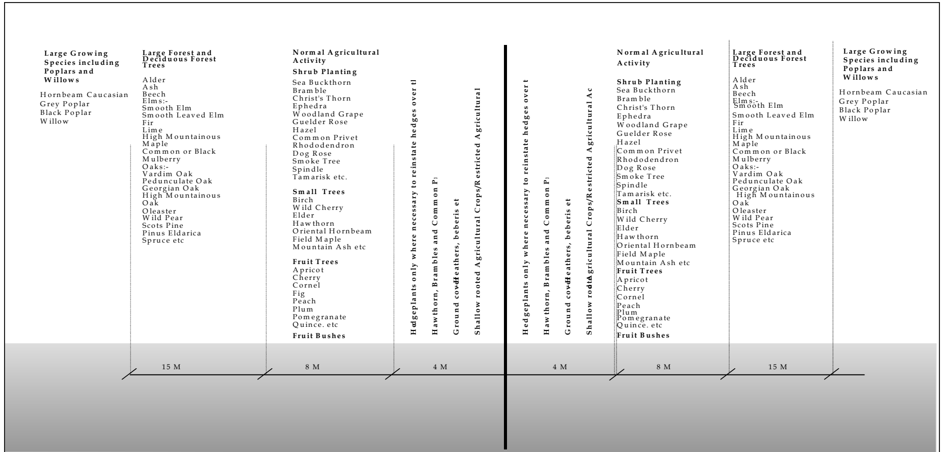
Figure 2.1 Tree Planting Across The Pipeline Corridor
